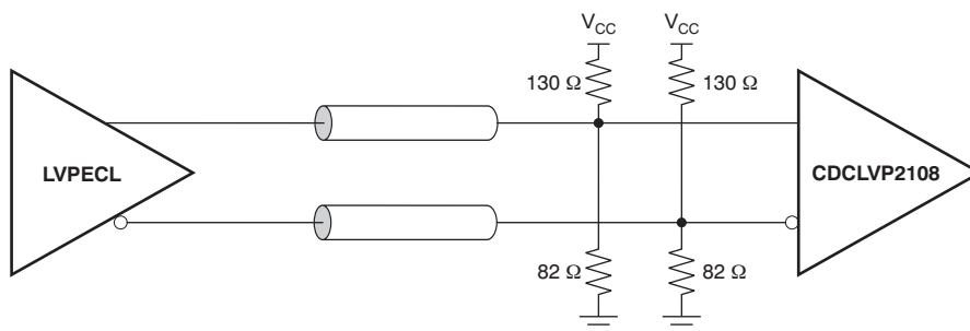
Figure 19. DC-Coupled LVPECL Inputs to CDCLVP2108 ( V_{CC} = 3.3\text{ V} )
