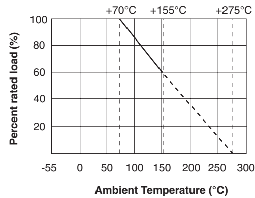
Derating Curve
