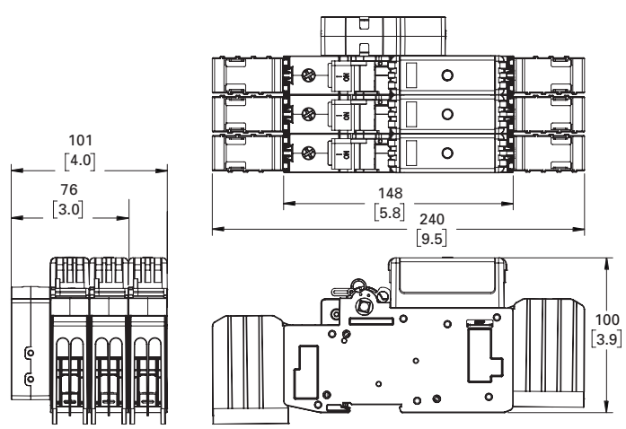
100 amp switches
