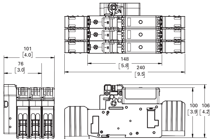
100 amp switches
