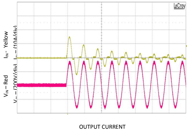
Figure 2. Inrush current V_{IN} = 230V_{AC} , 0° phase angle
