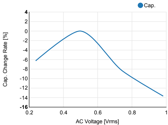
AC Voltage
