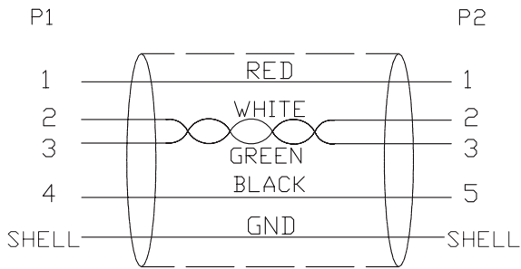
WIRE DIAGRAM
