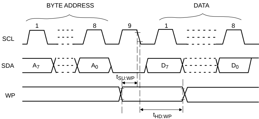
Figure 9. WP Timing
