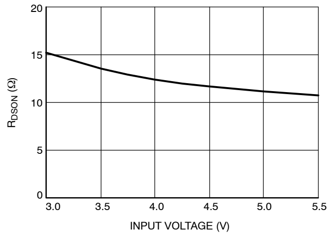
Figure 7. FLAG RDS(on) vs. Input Voltage
