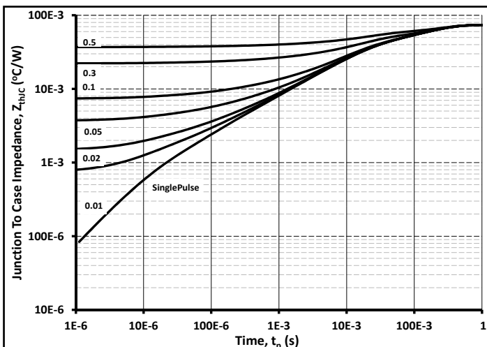
Figure 27. MOSFET Junction to Case Thermal Impedance
