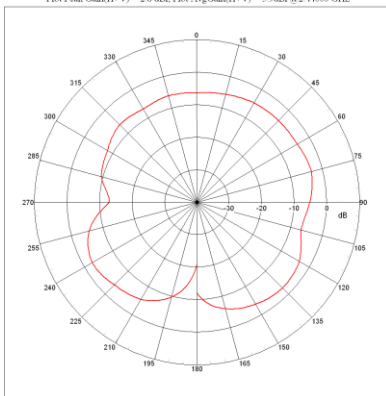
Far-field Power Distribution(H+V) on Y-Z Plane Plot Peak Gain(H+V)=-1.6 dB, Plot AvgGain(H+V)=-4.7dB @2.44000 GHz
