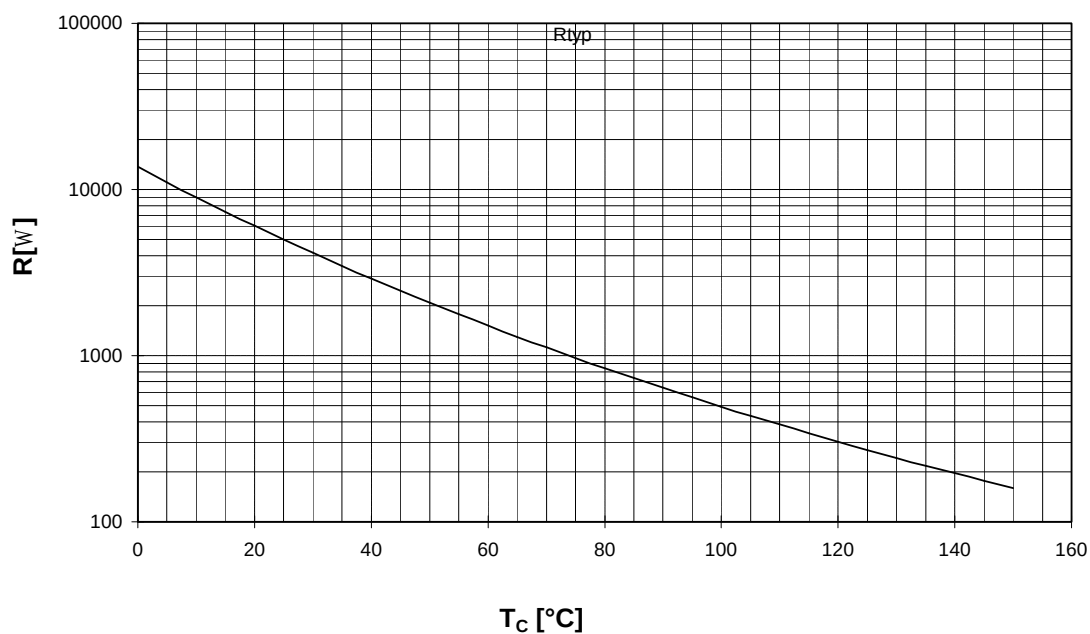
NTC- temperature characteristic (typical)
