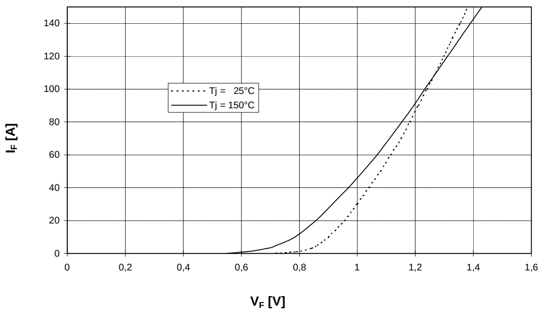
Forward characteristic of Rectifier Diode (typical)
