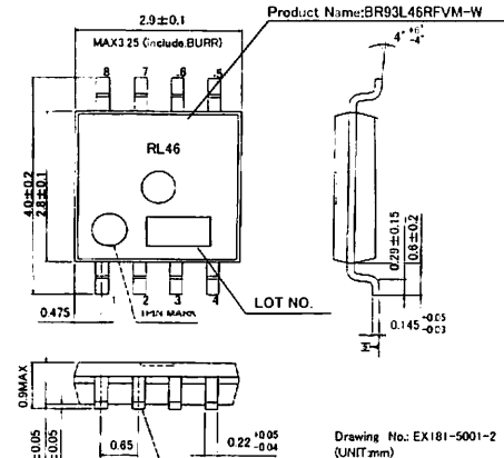
Fig.4-(b) PHYSICAL DIMENSION MSOP8 (BR93L46RFVM-W)
