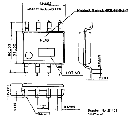
Fig.4-(f) PHYSICAL DIMENSION SOP-J8 (BR93L46RFJ-W)
