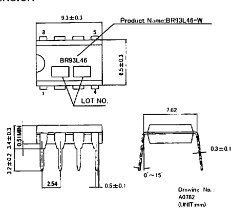
Fig.4-(a) PHYSICAL DIMENSION DIP8 (BR93L46-W)
