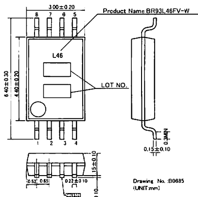
Fig.4-(g) PHYSICAL DIMENSION SSOP-B8 (BR93L46FV-W)
