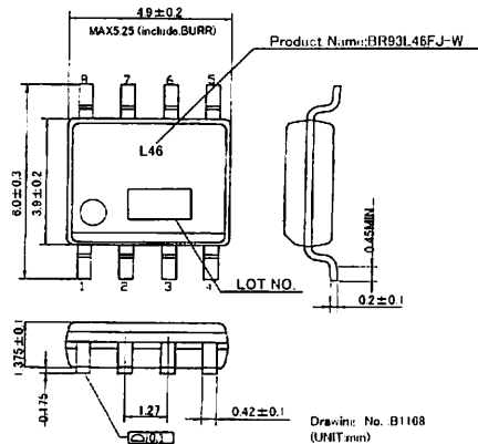
Fig.4-(e) PHYSICAL DIMENSION SOP-J8 (BR93L46FJ-W)
