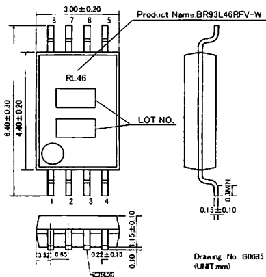
Fig.4-(h) PHYSICAL DIMENSION SSOP-B8 (BR93L46RFV-W)
