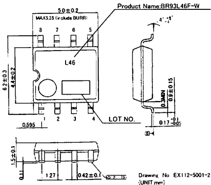
Fig.4-(c) PHYSICAL DIMENSION SOP8 (BR93L46F-W)
