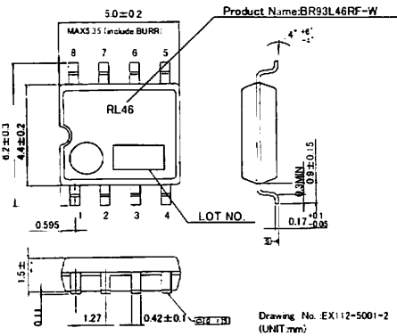
Fig.4-(d) PHYSICAL DIMENSION SOP8 (BR93L46RF-W)
