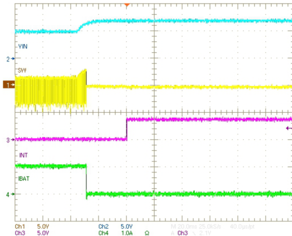
Figure 41. Input OVP Event With INT
