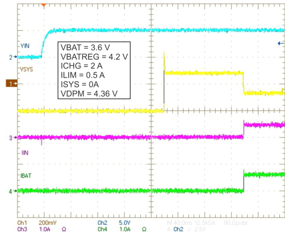
Figure 42. Start-up, 4.2 V
