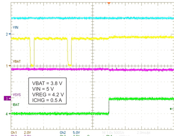
Figure 30. Battery Detection
