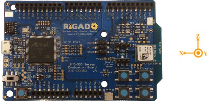
Figure 8: BMD-300 evaluation kit X-Y-Z orientation
