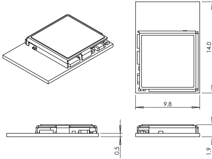
Figure 4: BMD-300 mechanical drawing
