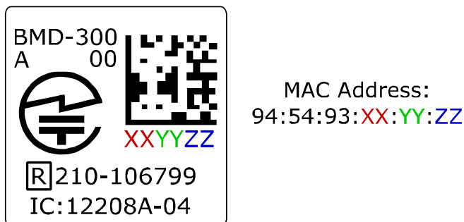
Figure 3: MAC Address
