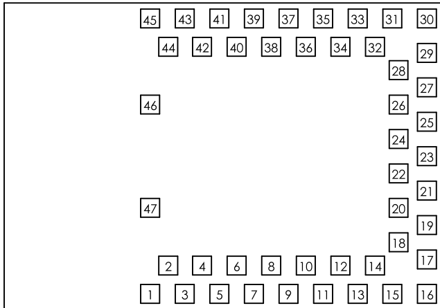
Figure 2: BMD-300 Pin assignment
