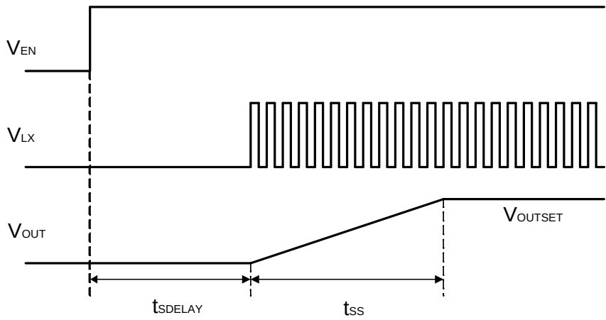
Figure 43. Timing Chart
