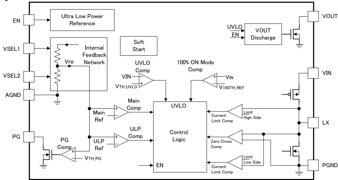
Figure 3. Block Diagram
