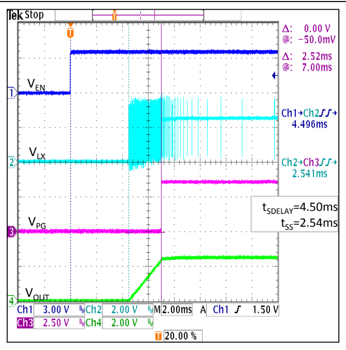
Figure 35. Startup ( V_{IN}=3.6\text{V} , V_{OUT}=2.5\text{V} , I_{OUT}=0\text{mA} , EN=0 \rightarrow V_{IN} )
