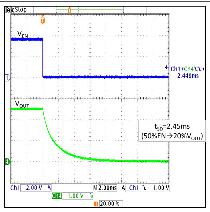
Figure 37. Shutdown ( V_{IN}=3.6\text{V} , V_{OUT}=2.5\text{V} , I_{OUT}=0\text{mA} , EN=V_{IN} \rightarrow 0 )
