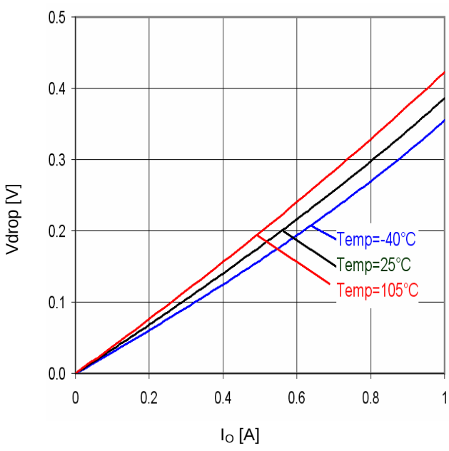
Fig.36 Minimum dropout Voltage 2 (V CC =4V, Ta=25°C)
