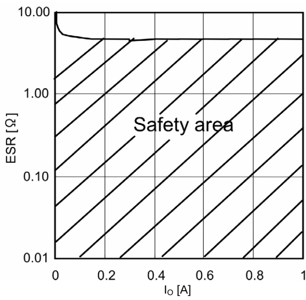
Fig.31 Operation Safety area
