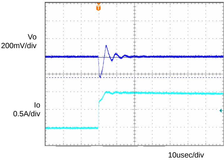
Fig.4 Transient Response (1.0→0A) Co=1 \mu F, Ta=25°C
