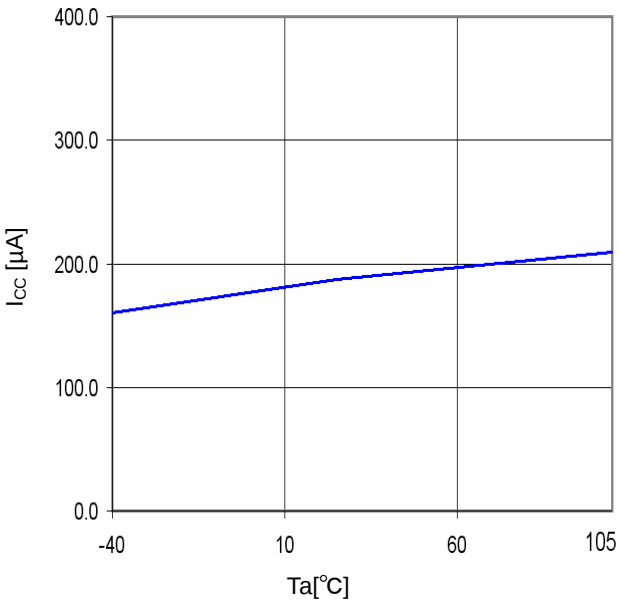
Fig.22 T_a - I_{cc}
