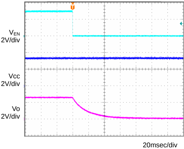
Fig.18 OFF sequence 2 C_o=1\mu F, T_a=-40^{\circ}C
