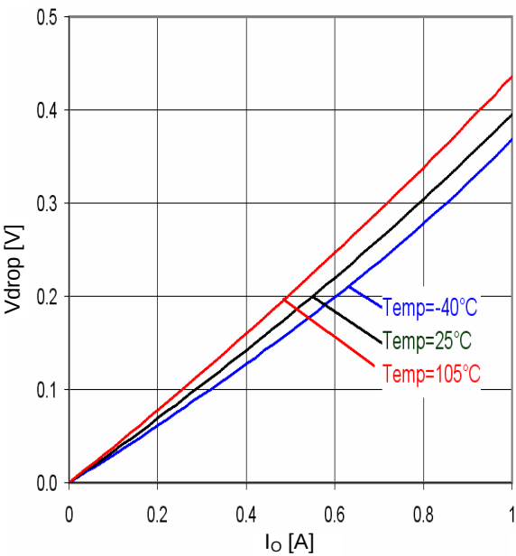
Fig.37 Minimum dropout Voltage 5 (V CC =5.5V, Ta=25°C)
