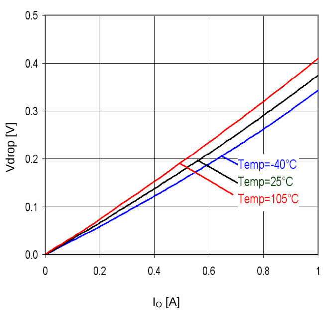
Fig.34 Minimum dropout Voltage 2 (Vcc=2.4V, Ta=25°C)
