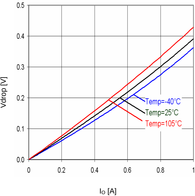
Fig.35 Minimum dropout Voltage 2 (V CC =3.3, Ta=25°C)
