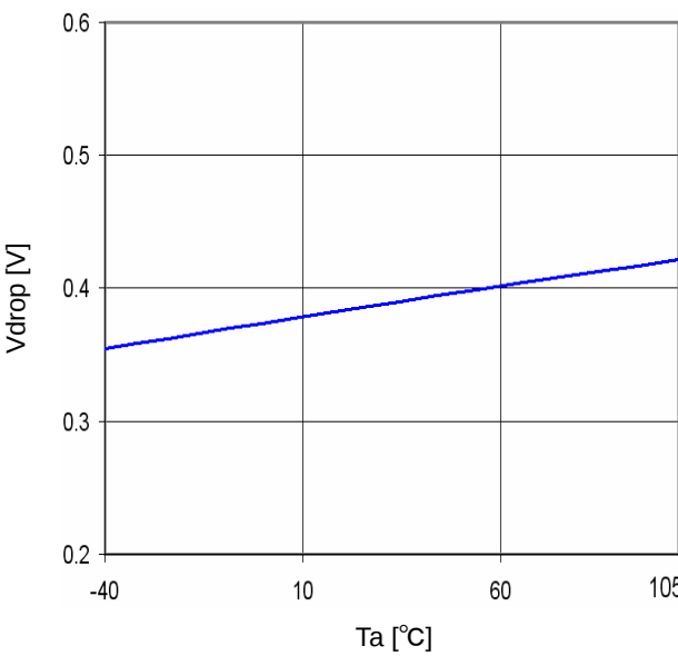
Fig.30 Minimum dropout Voltage1 ( V_{cc}=3.3\text{V} , I_o=1.0\text{A} )
