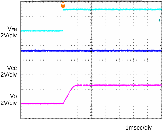
Fig.16 Input sequence 2 C_o=1\mu F, T_a=25^{\circ}C
