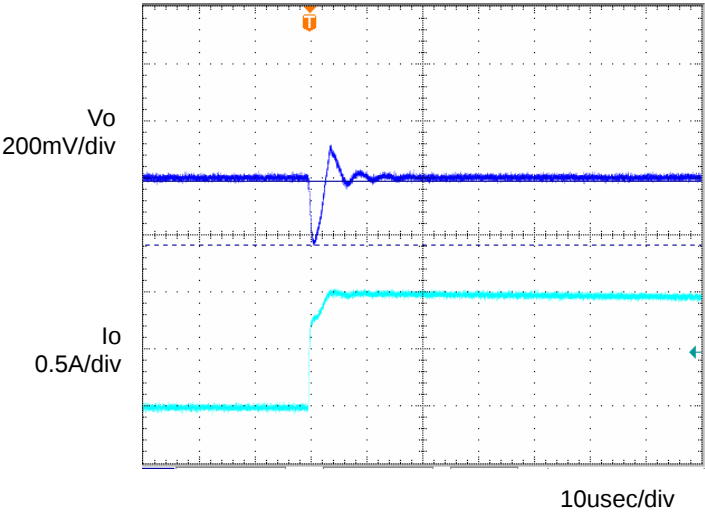
Fig.3 Transient Response (0→1.0A) Co=1 \mu F, Ta=-40°C
