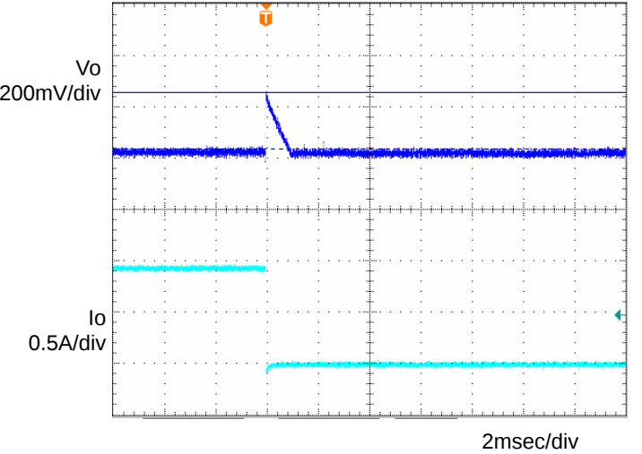
Fig.6 Transient Response (1.0 \rightarrow 0A) Co=1 \mu F, Ta=-40 ^{\circ} C
