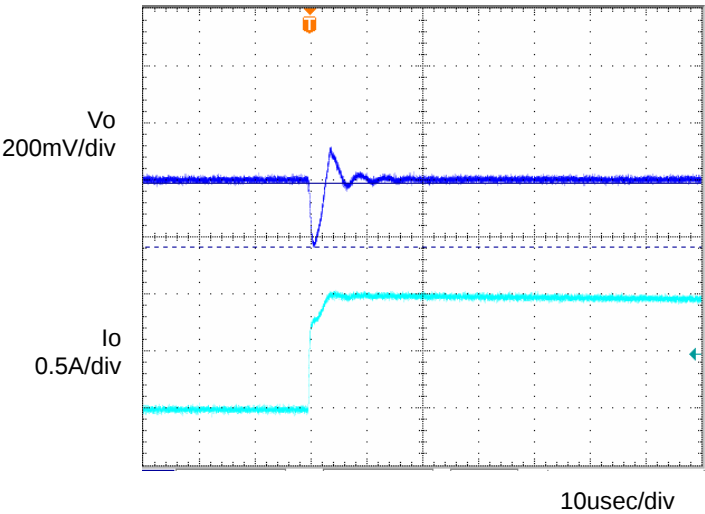
Fig.3 Transient Response (0 \rightarrow 1.0A) Co=1 \mu F, Ta=-40 ^{\circ} C
