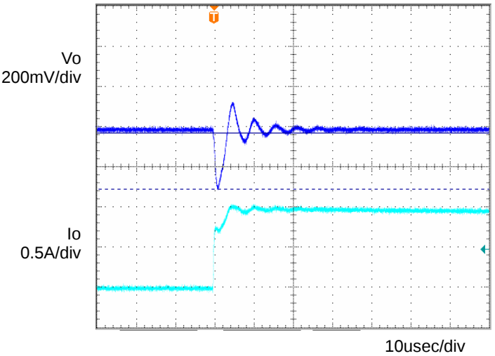
Fig.5 Transient Response (0 \rightarrow 1.0A) Co=1 \mu F, Ta=105 ^{\circ} C
