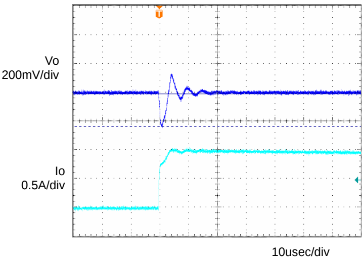
Fig.4 Transient Response (1.0 \rightarrow 0A) Co=1 \mu F, Ta=25 ^{\circ} C
