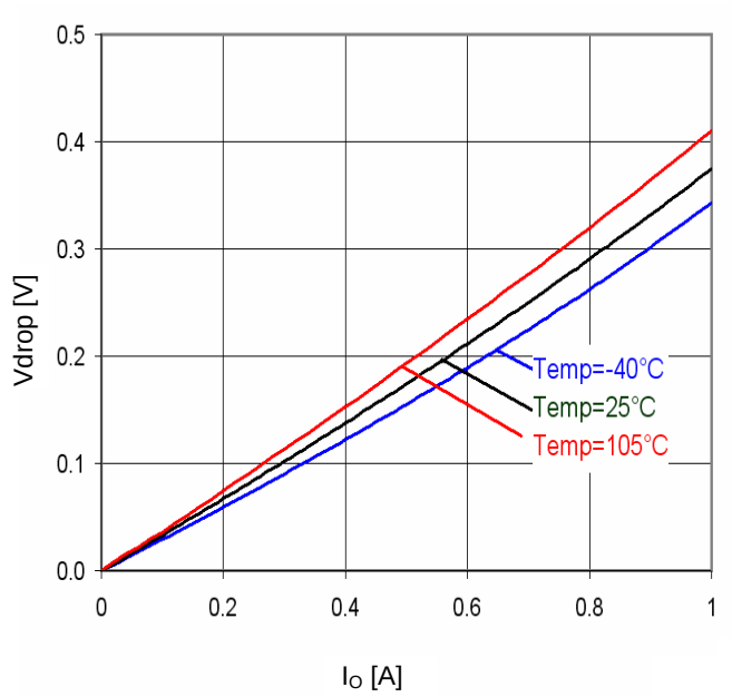
Fig.34 Minimum dropout Voltage 2 ( V_{CC}=2.4V , T_a=25^{\circ}C )
