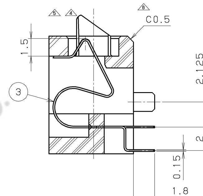
BB Section (S=5/1)
