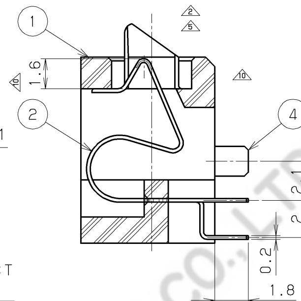
AA Section (S=5/1)
