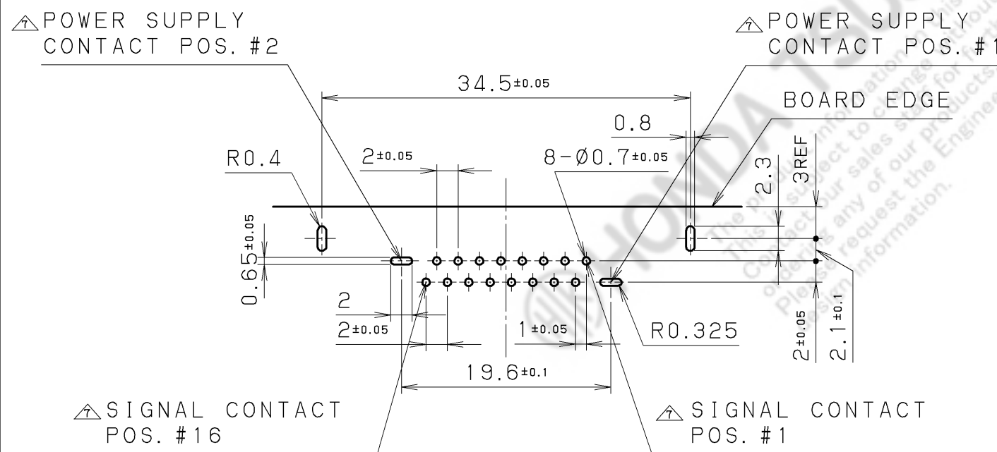
RECOMMENDED PCB LAYOUT (CONNECTOR SIDE) t=1.0
