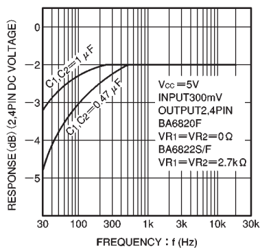
Fig. 10 Frequency characteristics
