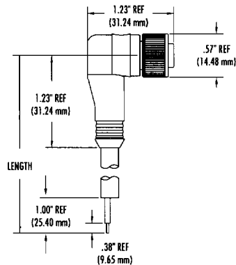
90° Female Plug
