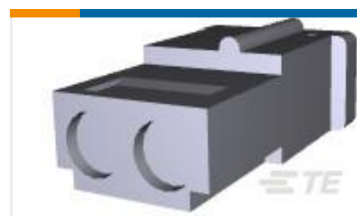
TE Part #1-480683-0 02P CMNL PLUG HSG F/H NATL
