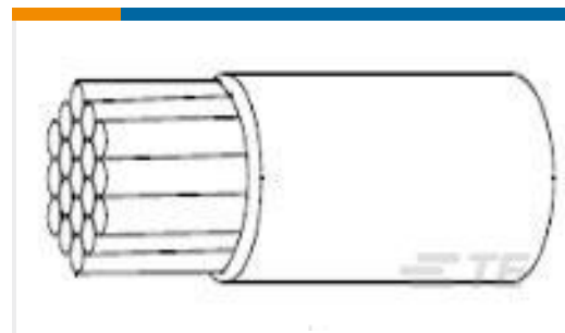
TE Part #129796-000 22759/33-24-3
