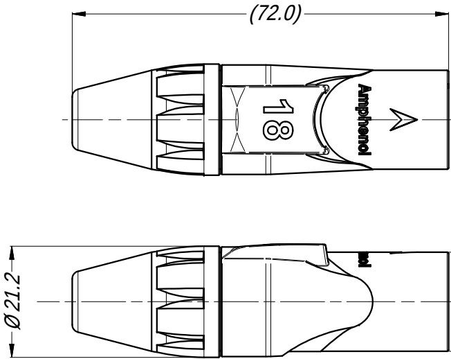
MALE CONNECTOR 1 : 1
