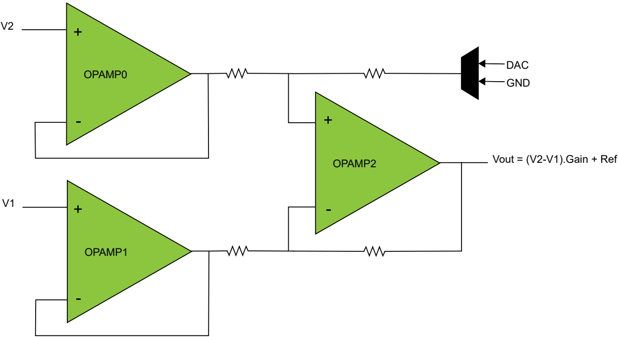
Figure 41-8. Instrumentation amplifier
