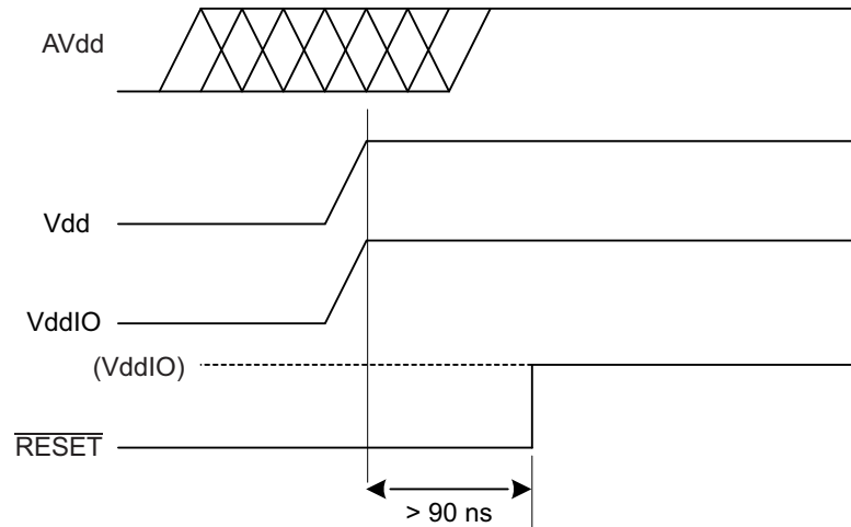
Figure 7-1. Power Sequencing on the mXT224T
