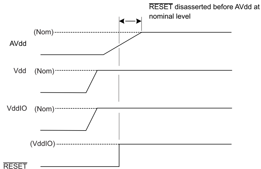
Figure 7-2. Power Sequencing on the mXT224T – Late rise on AVdd or XVdd
