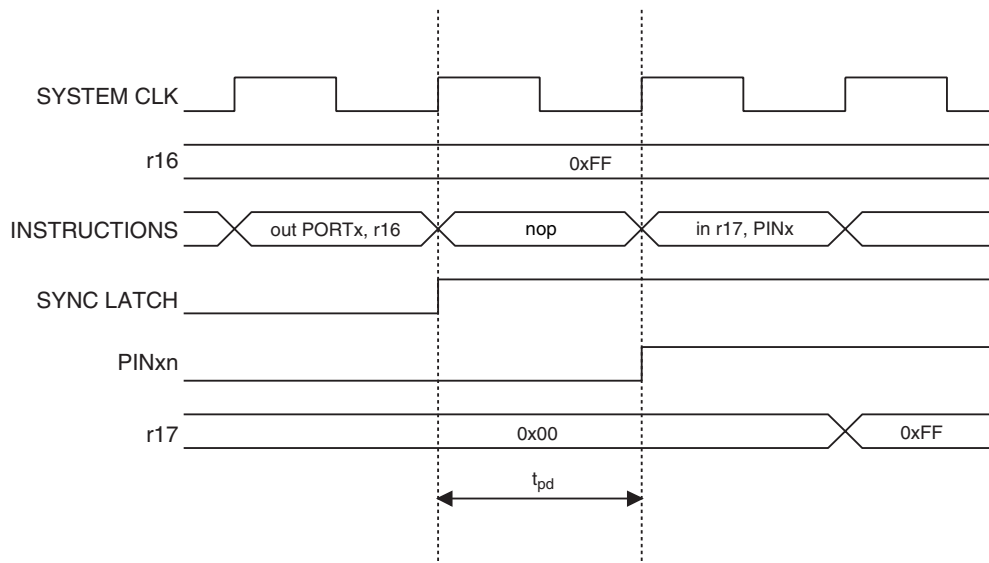
Figure 32. Synchronization when Reading a Software Assigned Pin Value
