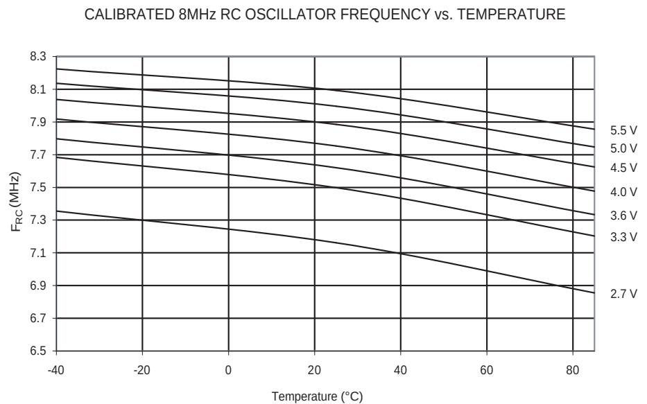
Figure 211. Calibrated 8 MHz RC Oscillator Frequency vs. Temperature
