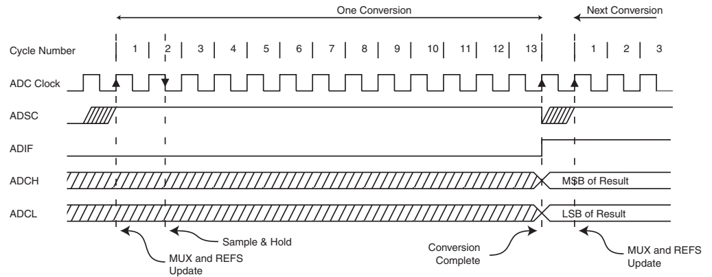
Figure 112. ADC Timing Diagram, Single Conversion
