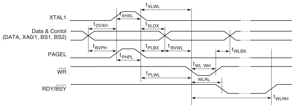
Figure 144. Parallel Programming Timing, Including some General Timing Requirements
