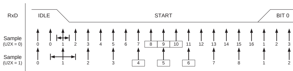
Figure 83. Start Bit Sampling
