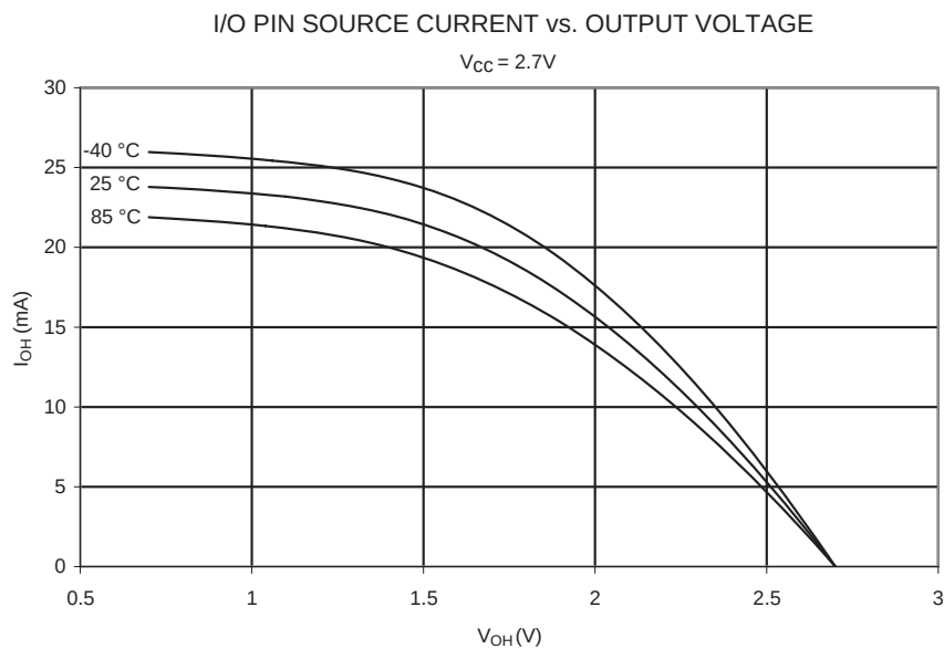
Figure 189. I/O Pin Source Current vs. Output Voltage ( V_{CC} = 2.7V )
