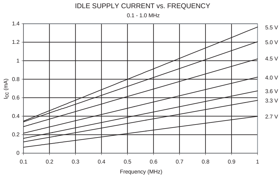
Figure 170. Idle Supply Current vs. Frequency (0.1 - 1.0 MHz)
