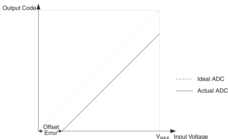
Figure 117. Offset Error
