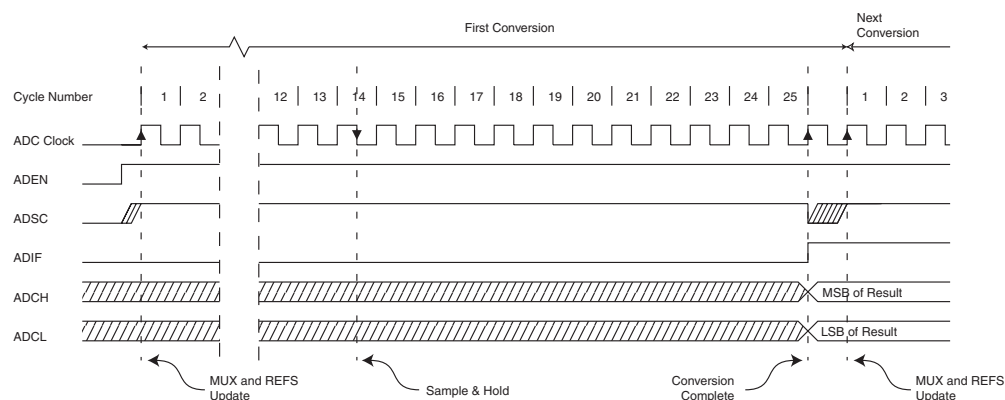
Figure 111. ADC Timing Diagram, First Conversion (Single Conversion Mode)
