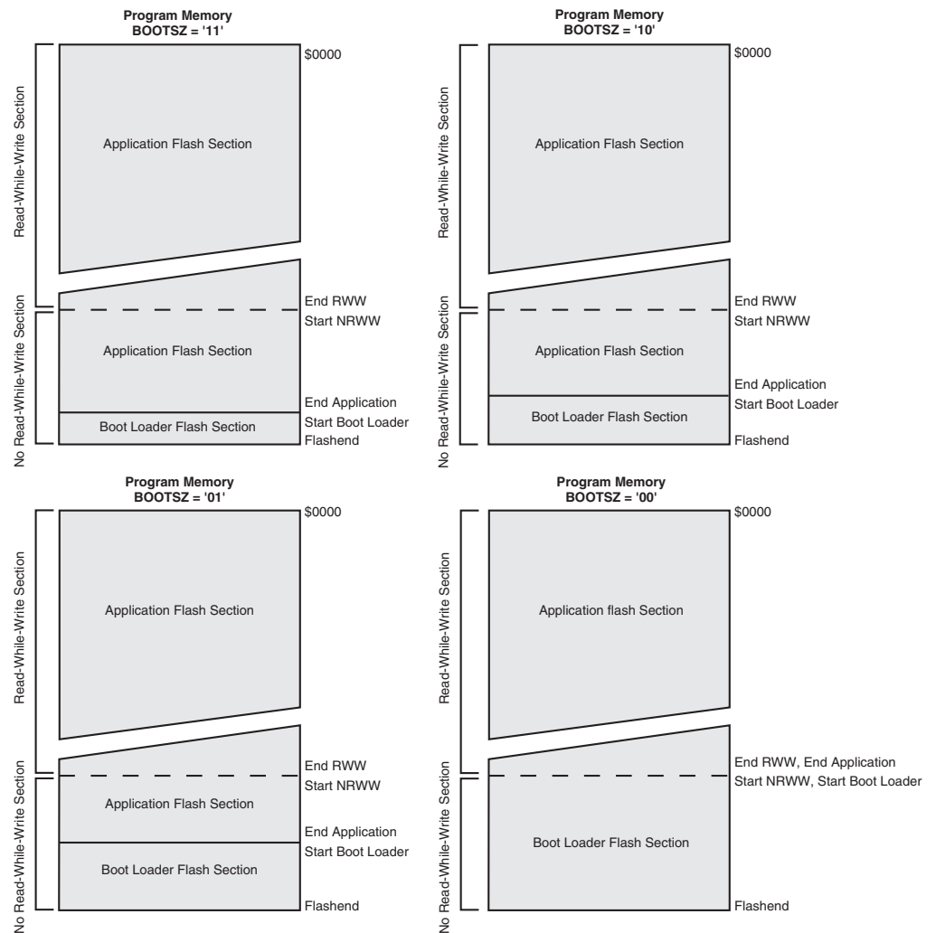
Figure 136. Memory Sections (1)
