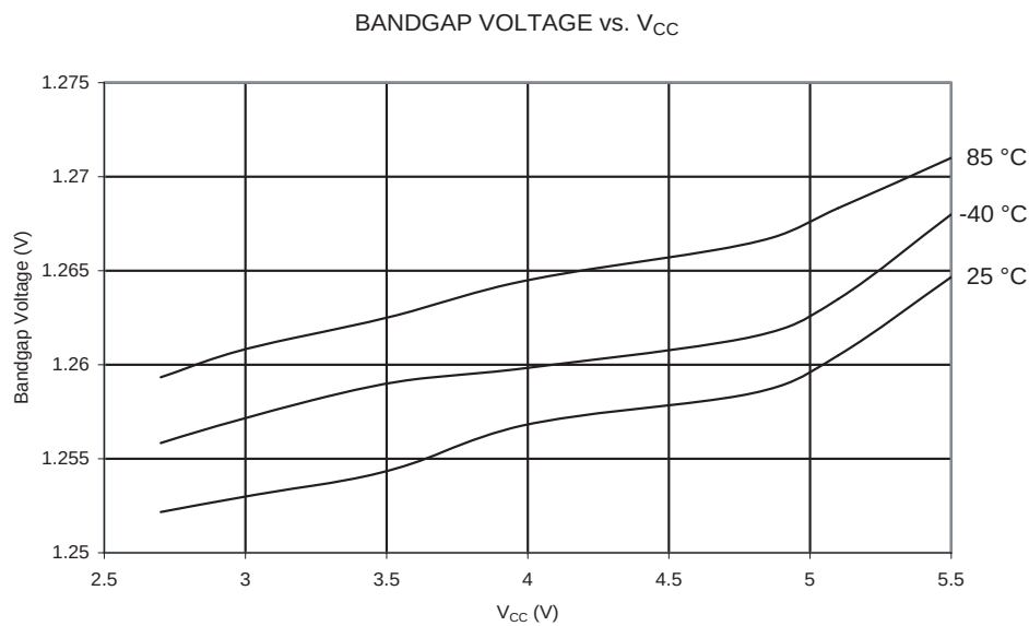
Figure 200. Bandgap Voltage vs. V_{CC}
