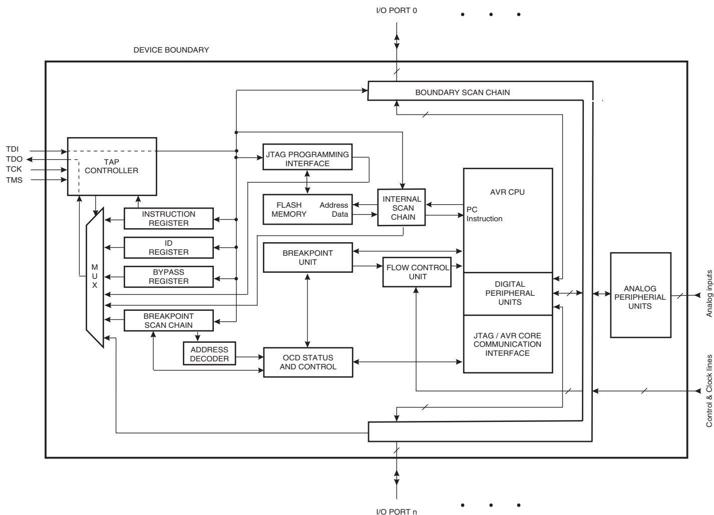
Figure 123. Block Diagram
