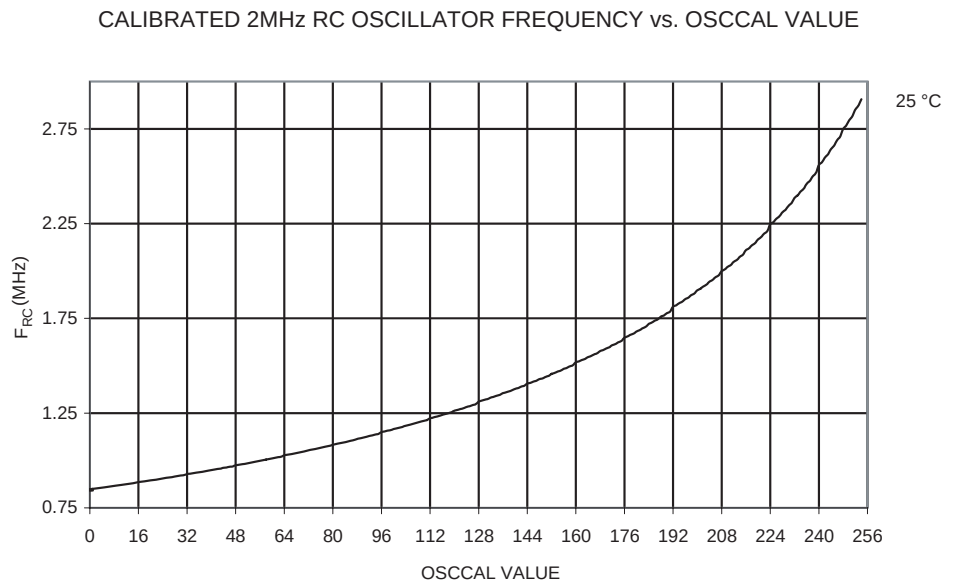
Figure 207. Calibrated 2 MHz RC Oscillator Frequency vs. OSCCAL Value
