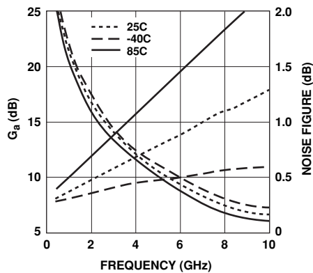
Figure 14. F_{min} and G_a vs. Frequency and Temp at V_{DS} = 4V , I_{DS} = 80\text{ mA} .
