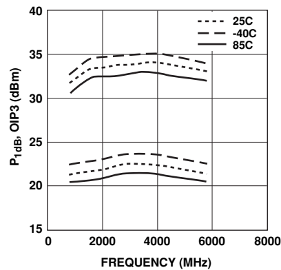
Figure 15. P_{1dB} , OIP3 vs. Frequency and Temp at V_{DS} = 4V , I_{DS} = 80\text{ mA} .
