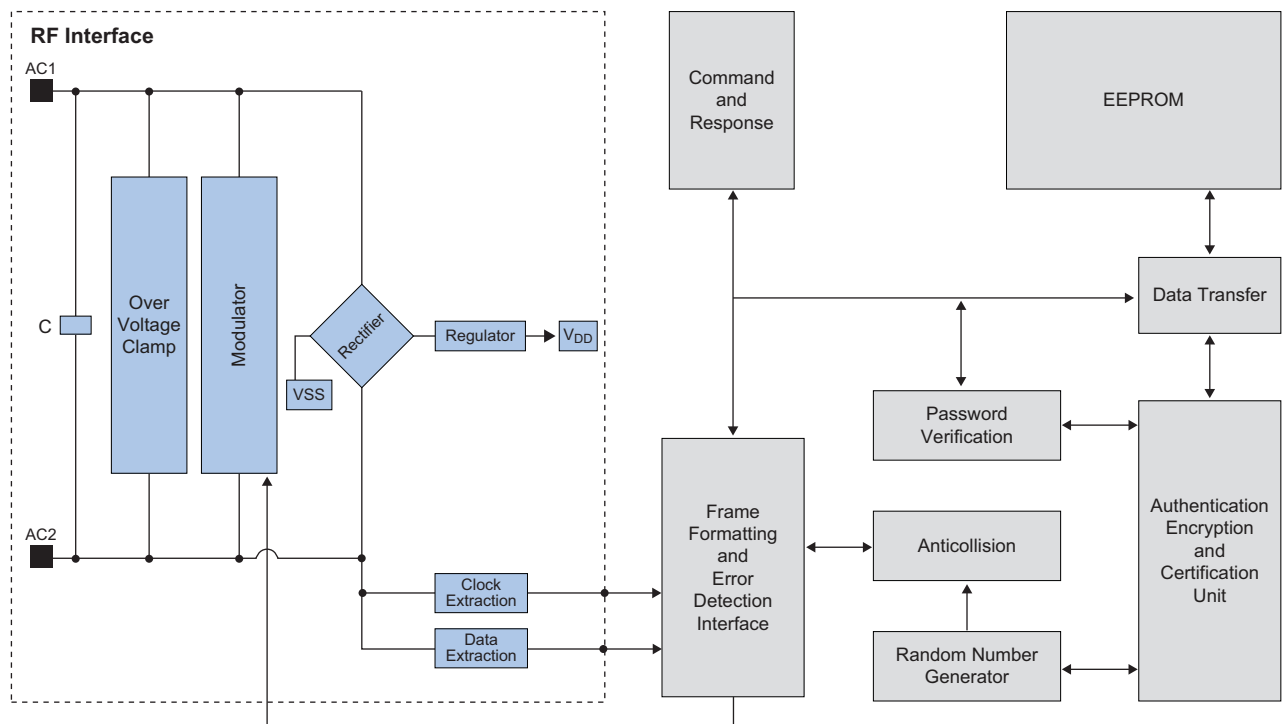
Figure 1-1. Block Diagram
