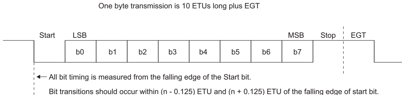
Figure O-1. Byte transmission format requirements for type B communications.
