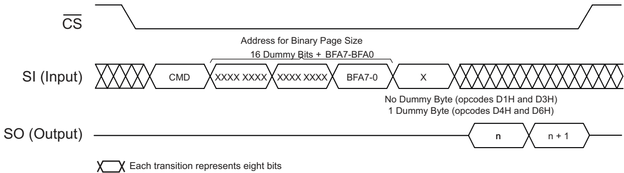
Figure 24-4. Buffer Read
