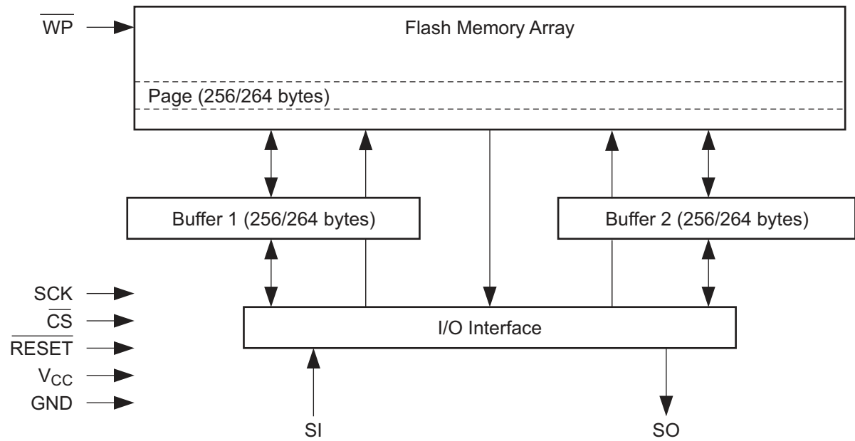
Figure 2-1. Block Diagram
