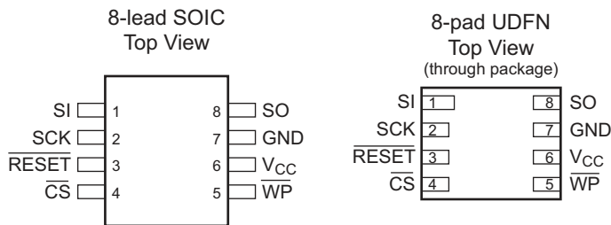
Figure 1-1. Pinouts
