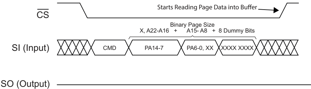
Figure 24-3. Main Memory Page to Buffer Transfer Data From the selected Flash Page is read into either SRAM Buffer
