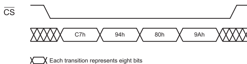
Figure 7-1. Chip Erase
