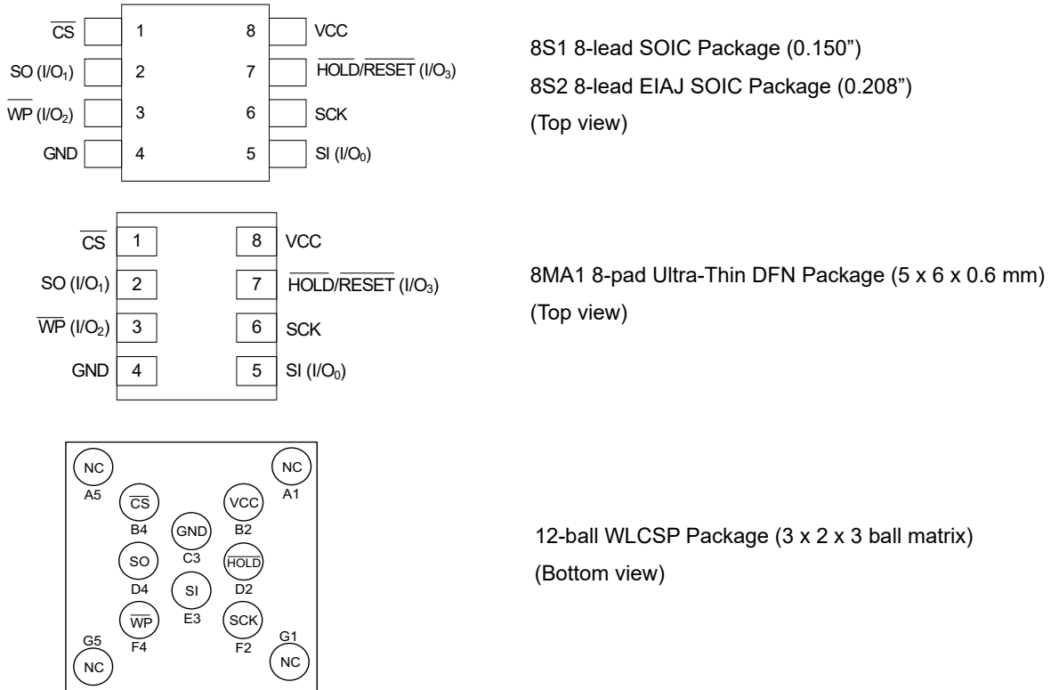
Figure 2. Memory Package Types
