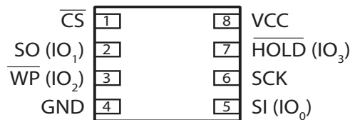
Figure 1-2. 8-UDFN (Top View)
