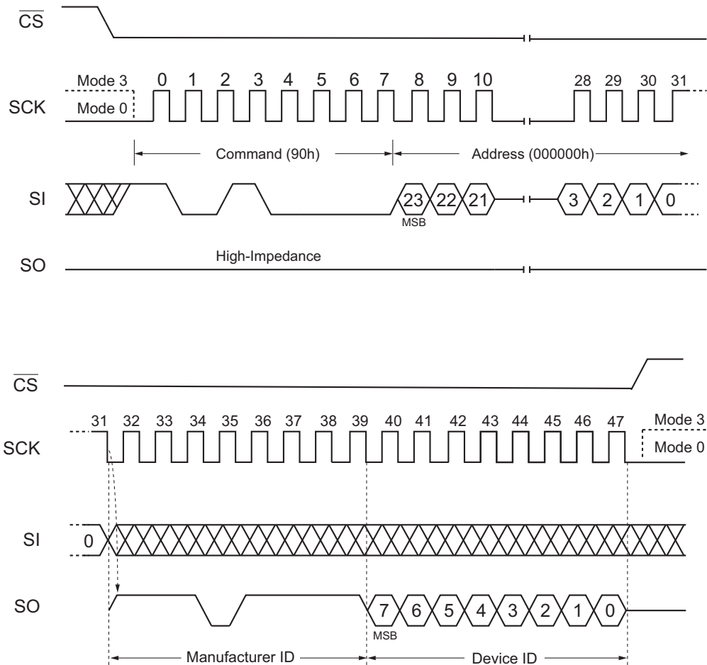
Figure 45. Read Manufacturer/ Device ID Command (SPI Mode)
