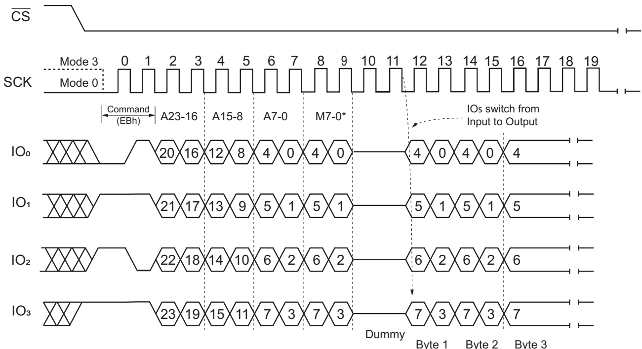
Figure 24. Fast Read Quad I/O Command (Initial command or previous M7-0 ≠ Axx, QPI mode)
