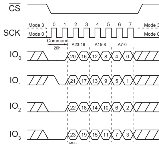
Figure 30. Block Erase Command (QPI Mode)
