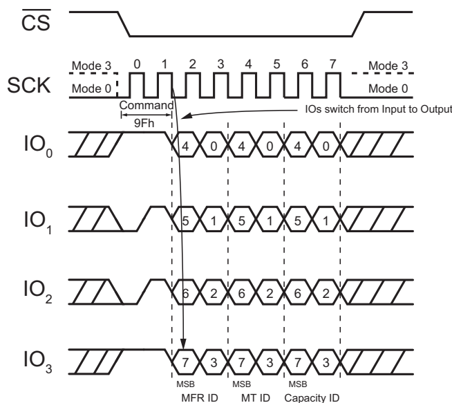
Figure 50. Read JEDEC ID Command (QPI Mode)
