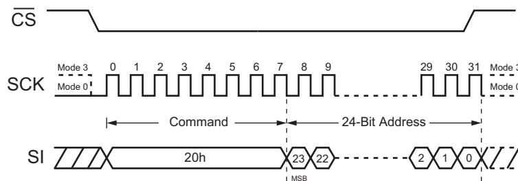
Figure 29. Block Erase Command (SPI Mode)
