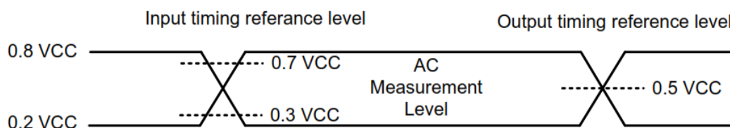
Figure 66. AC Measurement I/O Waveform
