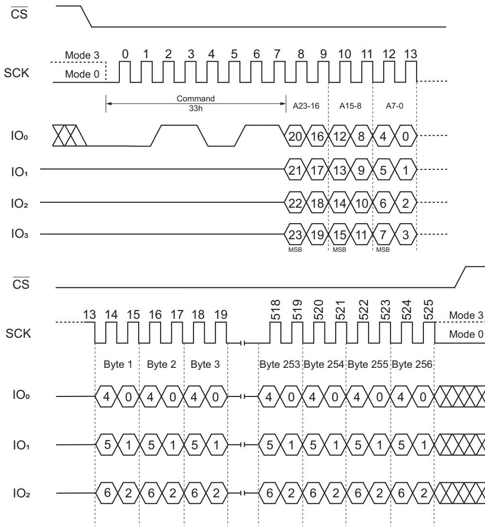
Figure 27. Quad Page Program Command (SPI mode)
