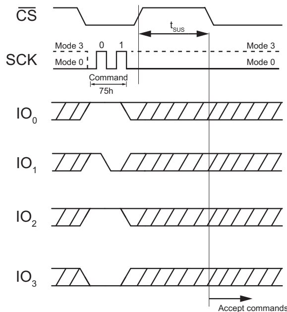
Figure 39. Erase / Program Resume Command (QPI Mode)
