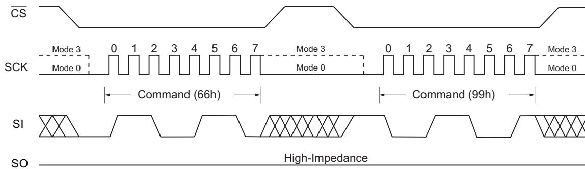
Figure 57. Enable Reset and Reset Command (SPI Mode)
