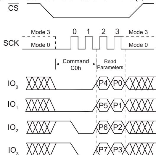
Figure 14. Set Read Parameters Command (QPI Mode)
