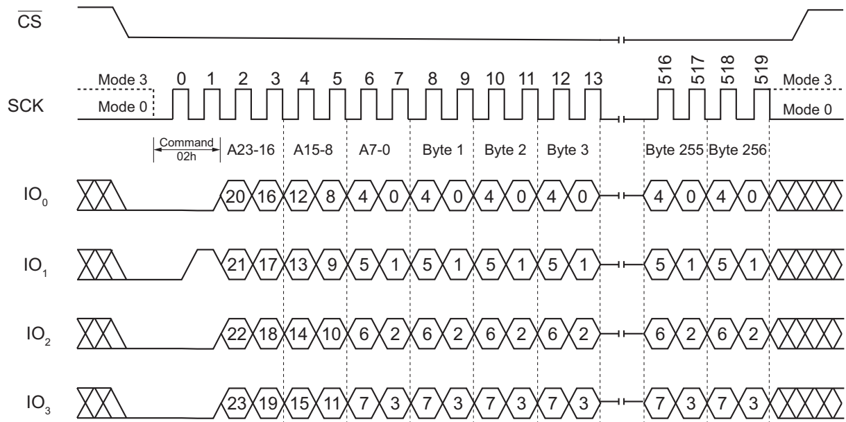
Figure 26. Page Program Command (QPI Mode)
