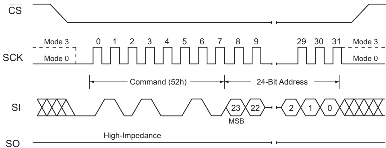
Figure 31. 32 kB Block Erase Command (SPI Mode)
