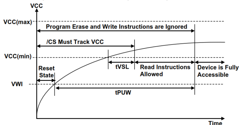
Figure 65. Power-Up Timing and Voltage Levels
