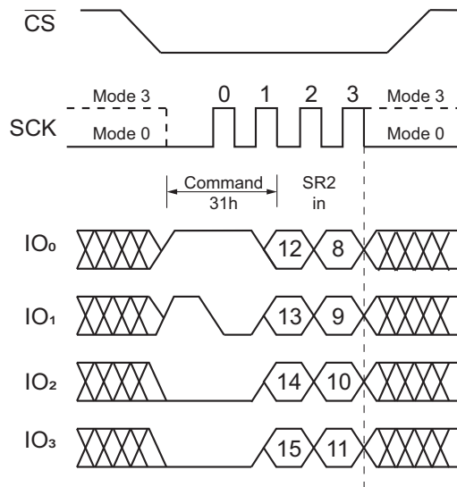
Figure 13. Write Status Register-2 Command (QPI Mode)
