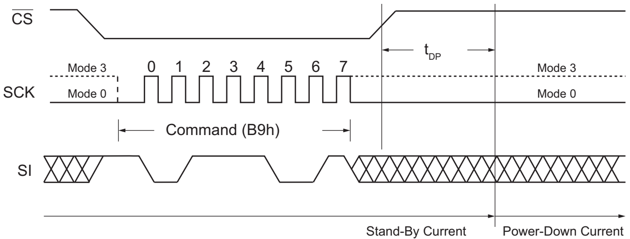
Figure 40. Deep Power-Down Command (SPI Mode)
