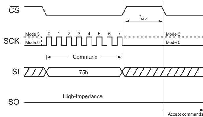
Figure 36. Erase Suspend Command (SPI Mode)
