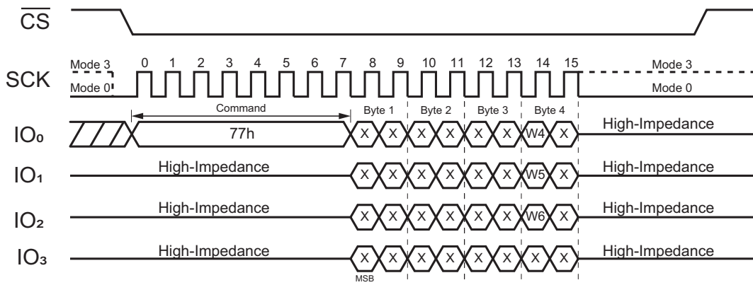
Figure 55. Set Burst with Wrap Command Sequence
