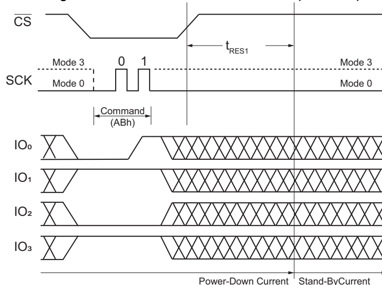
Figure 43. Release Power-Down Command (QPI Mode)
