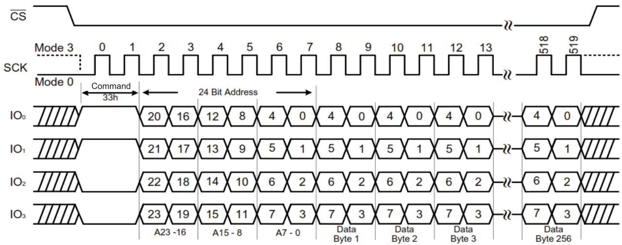
Figure 28. Quad Page Program Command (QPI mode)
