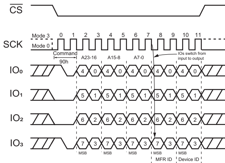
Figure 46. Read Manufacturer/ Device ID Command (QPI Mode)
