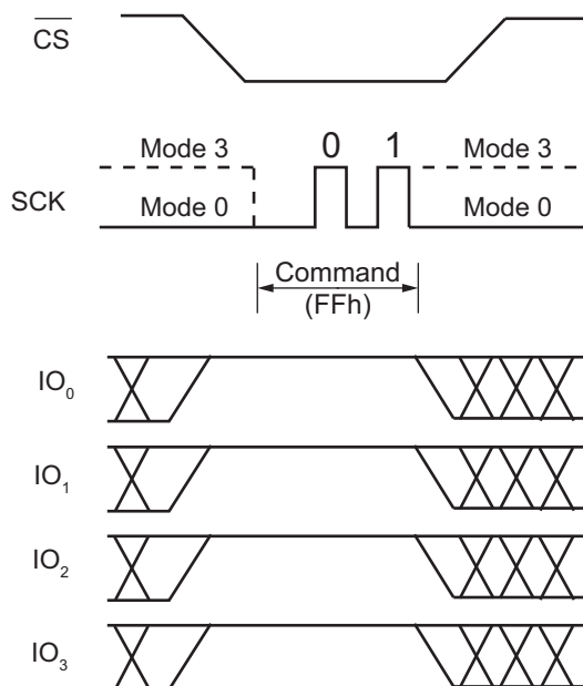
Figure 52. Disable QPI Command for QPI Mode
