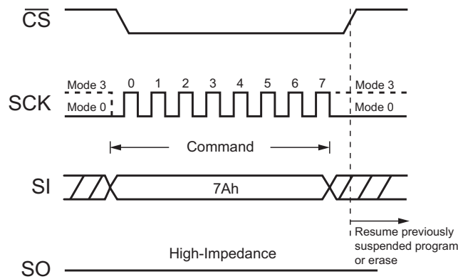
Figure 38. Erase / Program Resume Command (SPI Mode)
