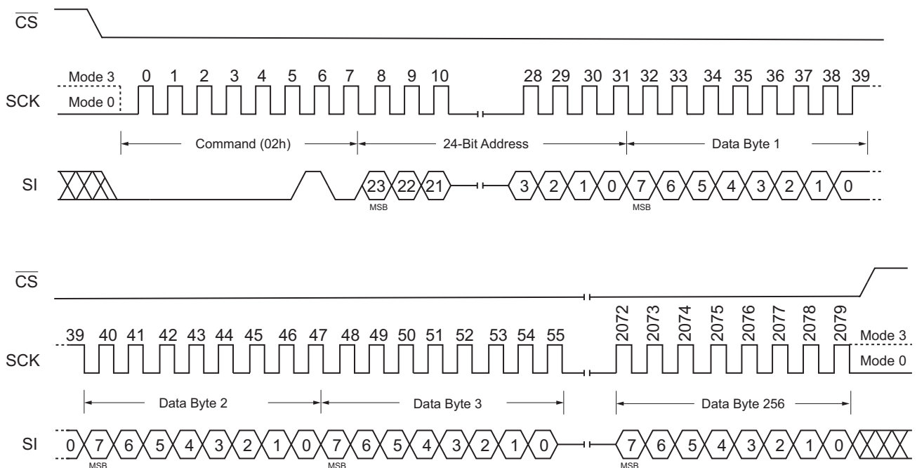
Figure 25. Page Program Command (SPI Mode)
