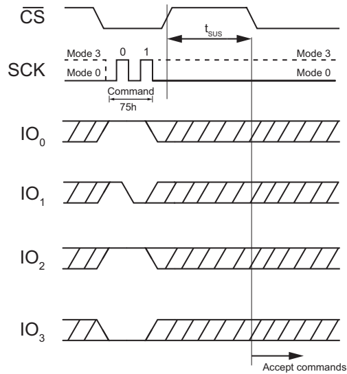
Figure 37. Erase Suspend Command (QPI Mode)
