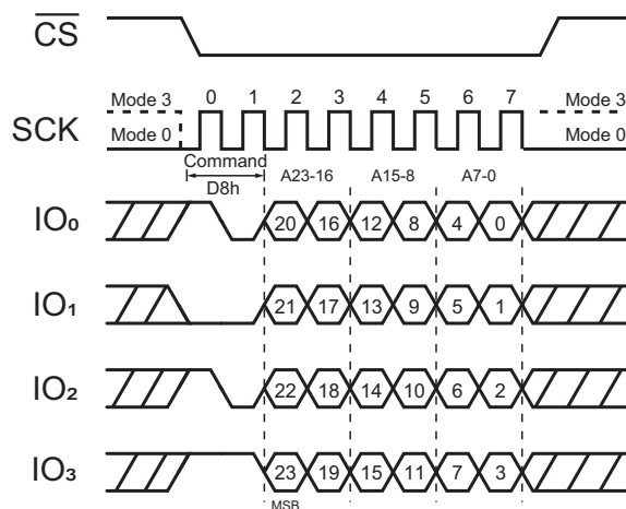
Figure 34. 64 kByte Block Erase Command (QPI Mode)
