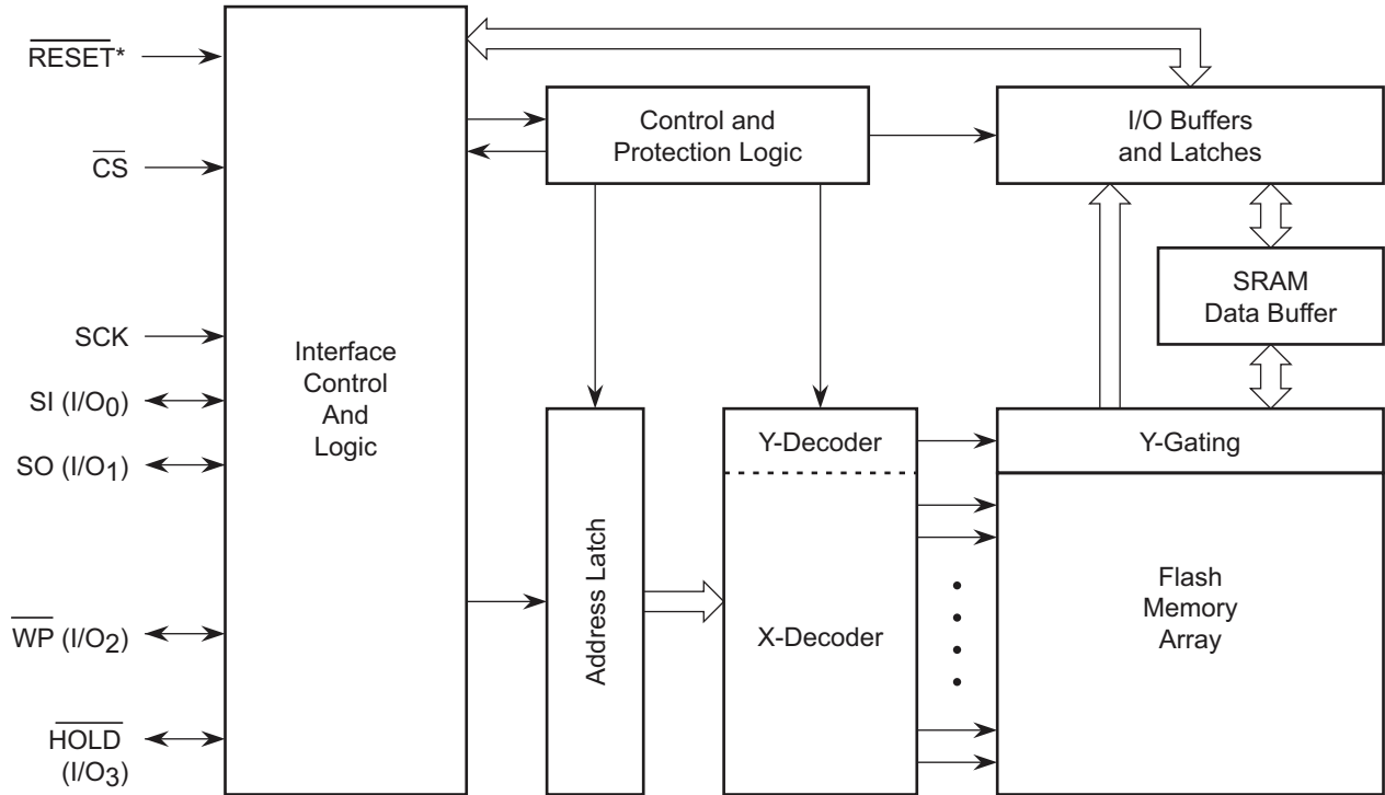
Figure 3. AT25QL641 Block Diagram
