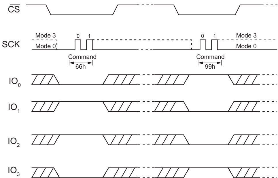
Figure 58. Enable Reset and Reset Command (QPI Mode)
