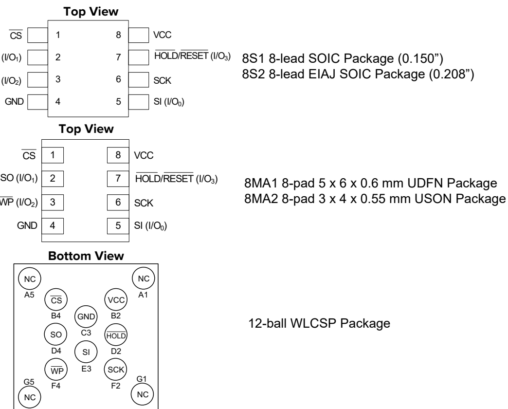
Figure 2. Memory Package Types
