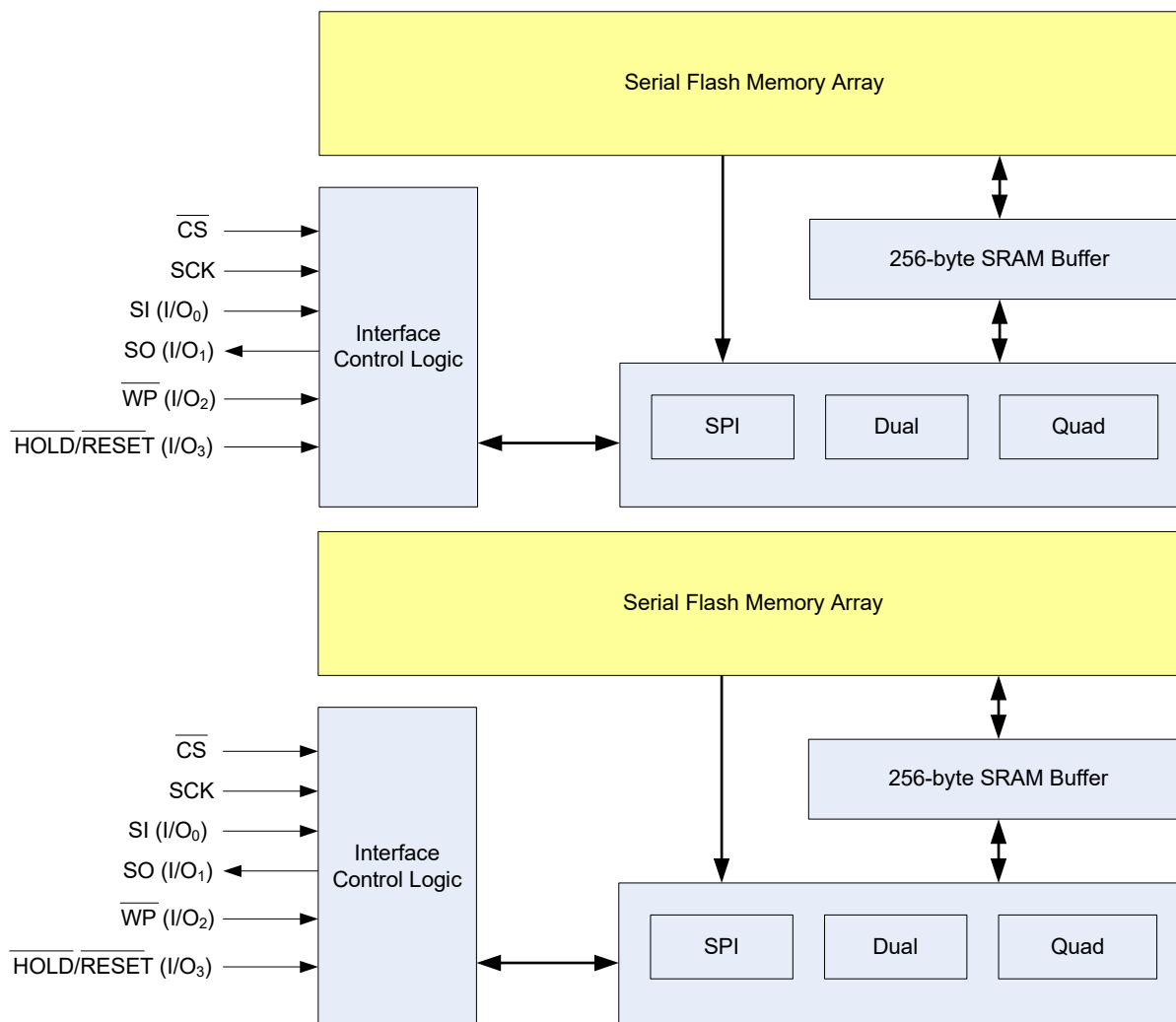
Figure 1. Block Diagram
