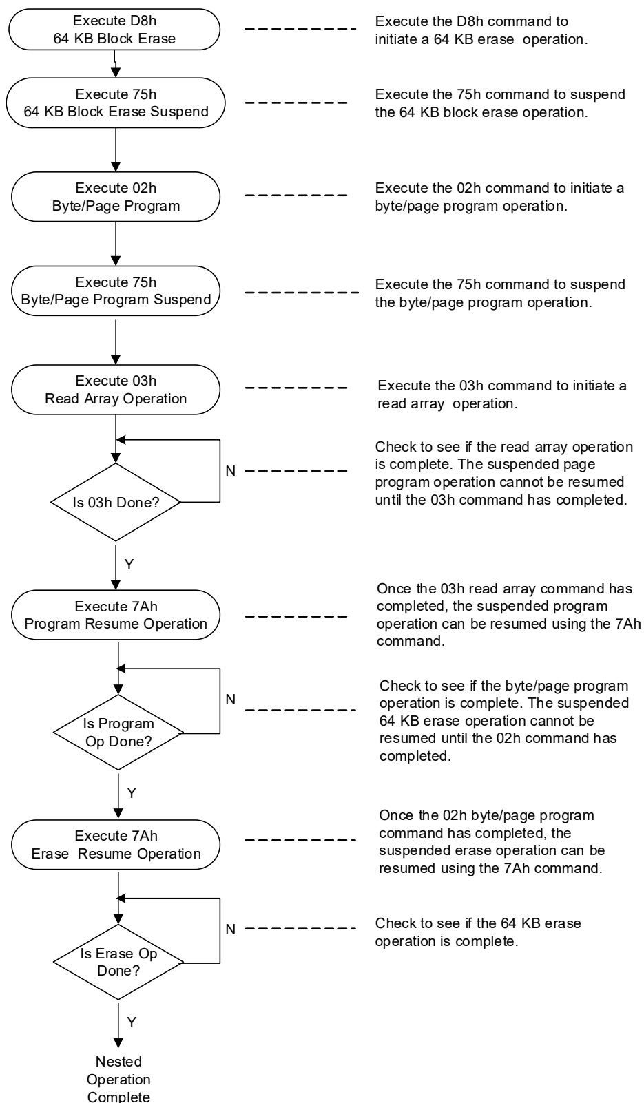
Figure 20. Flow Diagram of Nested Operations Example
