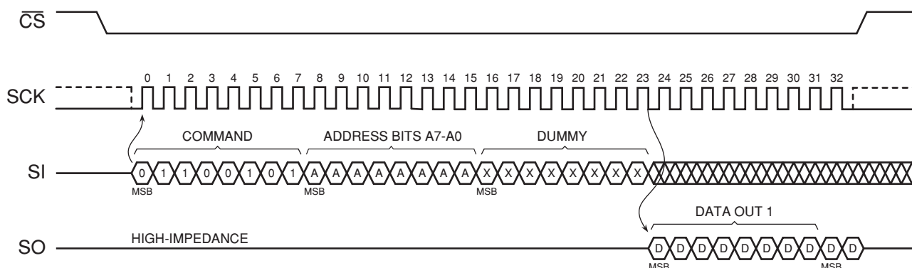
Figure 25. Status Register Read Operation Showing 8-bit Address Field
