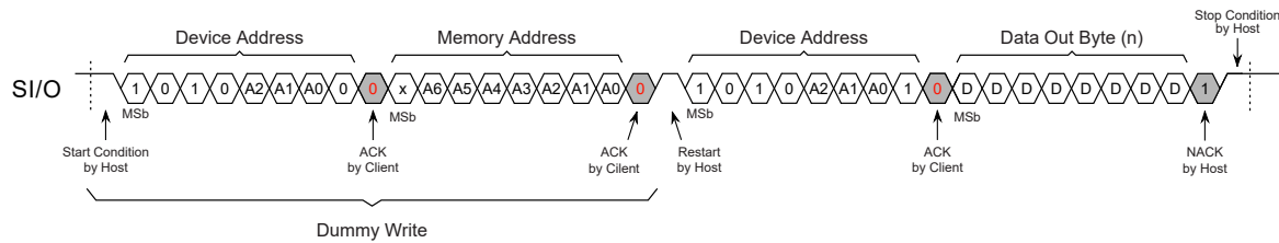
Figure 8-2. Random Read
