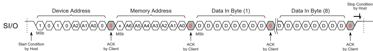
Figure 7-2. Page Write
