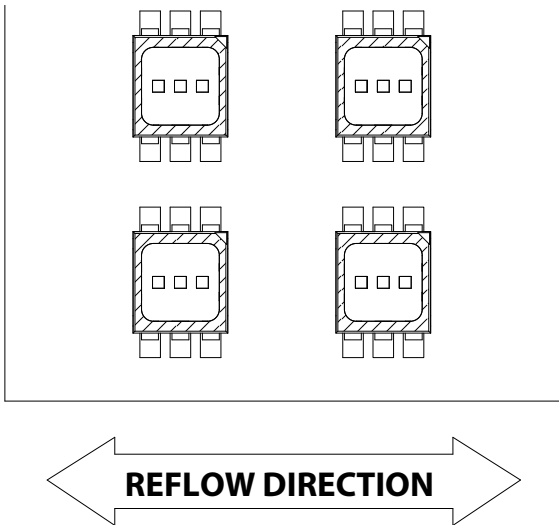
Figure 22: Board Reflow Direction
