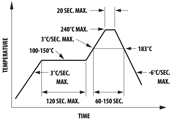
Figure 20: Leaded Reflow Soldering
