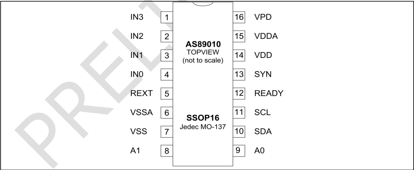
Figure 16: Pin configuration
