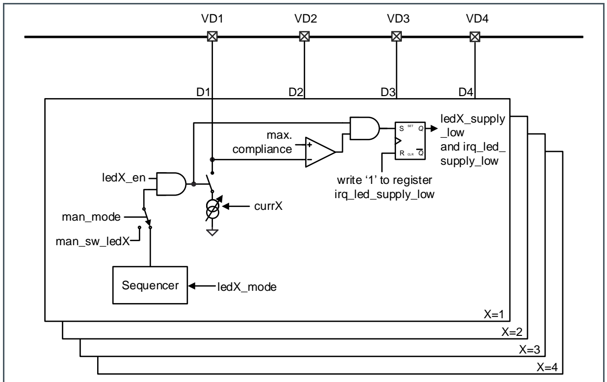
Figure 10: LED Drivers
