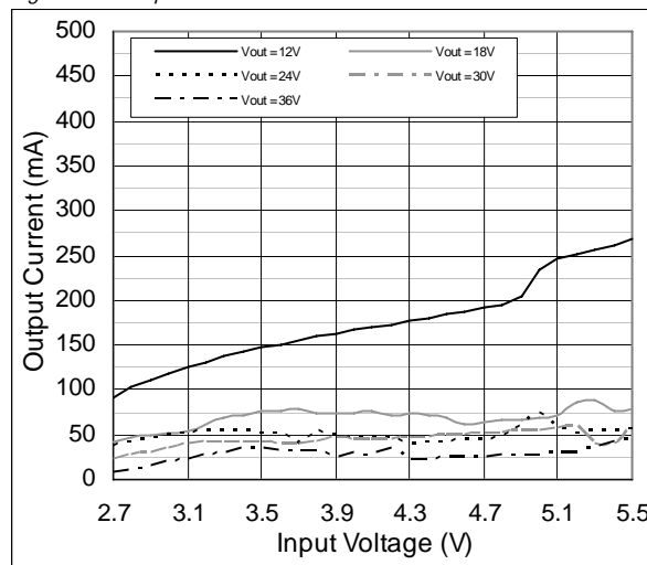
Figure 14. Output Current vs. V_{IN}
