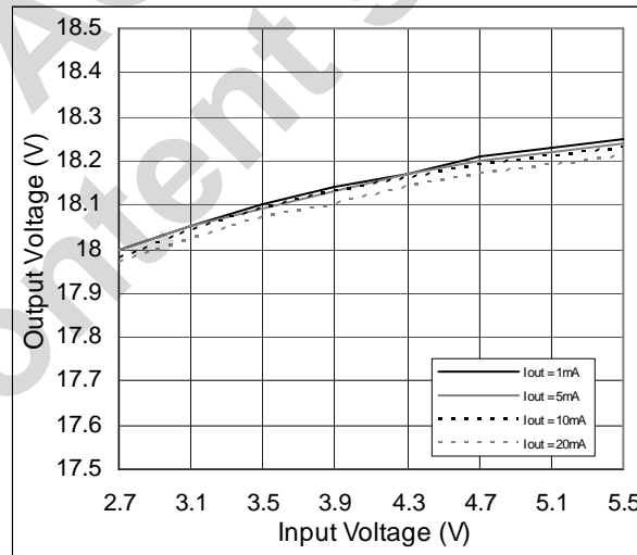
Figure 12. Output Voltage vs. Input Voltage; V_{OUT} = 18V
