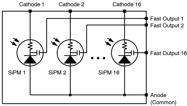
Figure 2. Array Schematic Showing Pixel Connections
