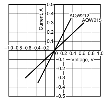
8.-(1) Voltage vs. current characteristics of output at MOS portion Measured portion: between terminals 5 and 6, 7 and 8; Ambient temperature: 25°C 77°F
