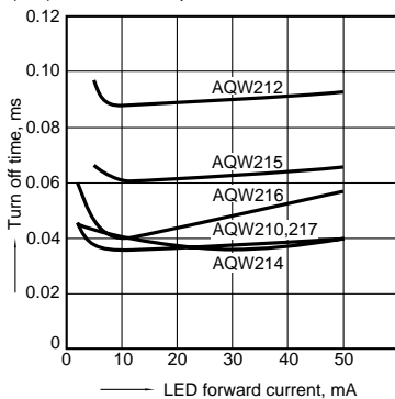
11. LED forward current vs. turn off time characteristics Measured portion: between terminals 5 and 6, 7 and 8; Load voltage: Max. (DC); Continuous load current: Max. (DC); Ambient temperature: 25°C 77°F
