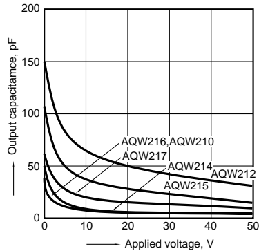
12. Applied voltage vs. output capacitance characteristics Measured portion: between terminals 5 and 6, 7 and 8; Frequency: 1 MHz; Ambient temperature: 25°C 77°F
