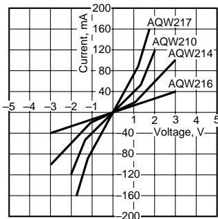
8.-(2) Voltage vs. current characteristics of output at MOS portion Measured portion: between terminals 5 and 6, 7 and 8; Ambient temperature: 25°C 77°F
