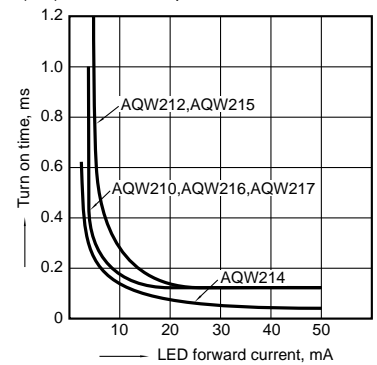
10. LED forward current vs. turn on time characteristics Measured portion: between terminals 5 and 6, 7 and 8; Load voltage: Max. (DC); Continuous load current: Max. (DC); Ambient temperature: 25°C 77°F
