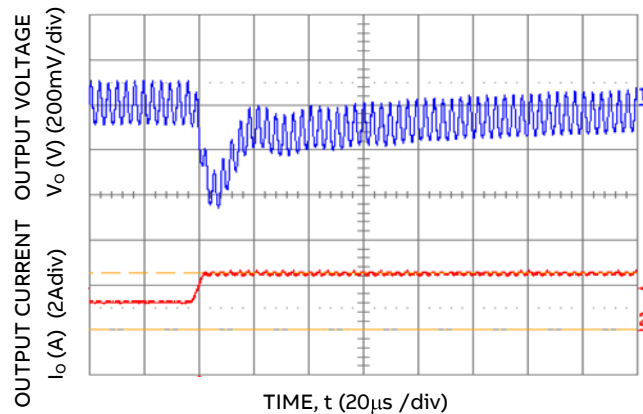
Figure 22. Transient Response to Dynamic Load Change from 50% to 100% at 28V in , C ext = 1x10µF ceramic, C Tune =150pF & R Tune =220Ω
