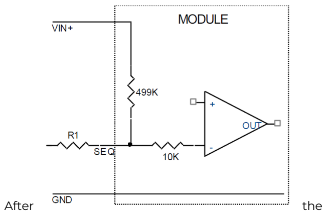
Figure 47. Circuit showing connection of the sequencing signal to the SEQ pin.
