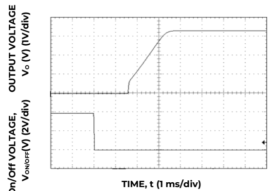
Figure 29. Typical Start-up Using On/Off Voltage ( I_O = I_{O, \text{max}} ).
