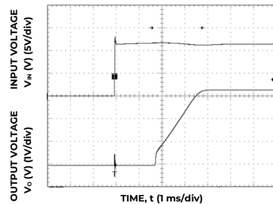
Figure 30. Typical Start-up Using Input Voltage ( V_{IN} = 12 \text{ V} , I_O = I_{O, \text{max}} ).
