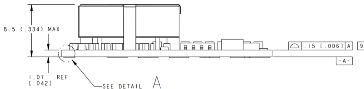
Side View
