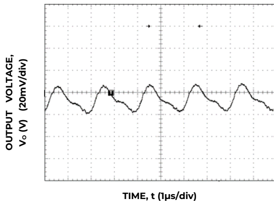
Figure 27. Typical Output Ripple and Noise, V_{IN} = 12 \text{ V} , I_O = I_{O, \text{max}} .
