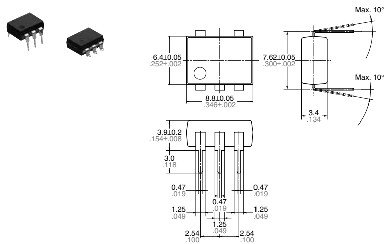
Through hole terminal type
