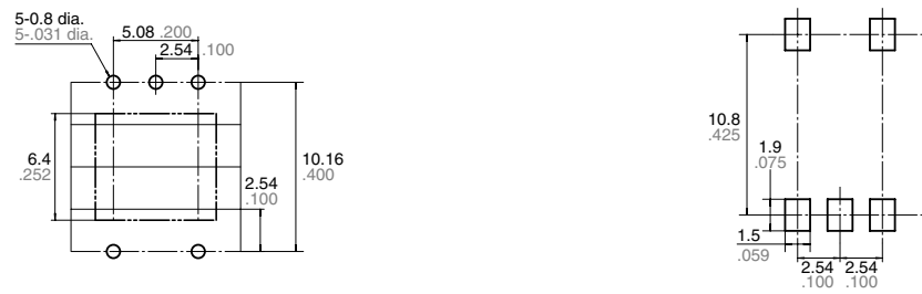
PC board pattern (BOTTOM VIEW)
