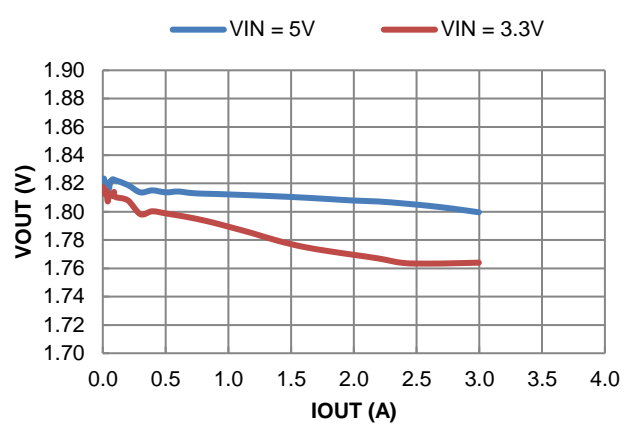
Figure 13. Load Regulation
