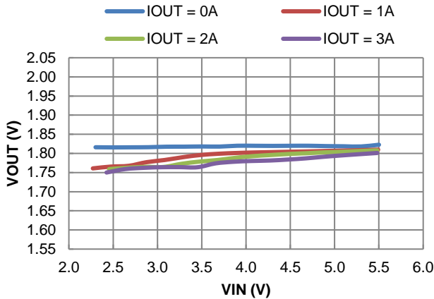
Figure 12. Line Regulation
