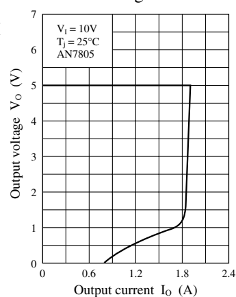
Current limiting characteristic
