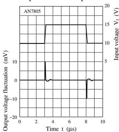
Input transient response
