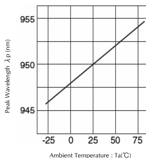
Ambient Temperature vs. Peak Wavelength
