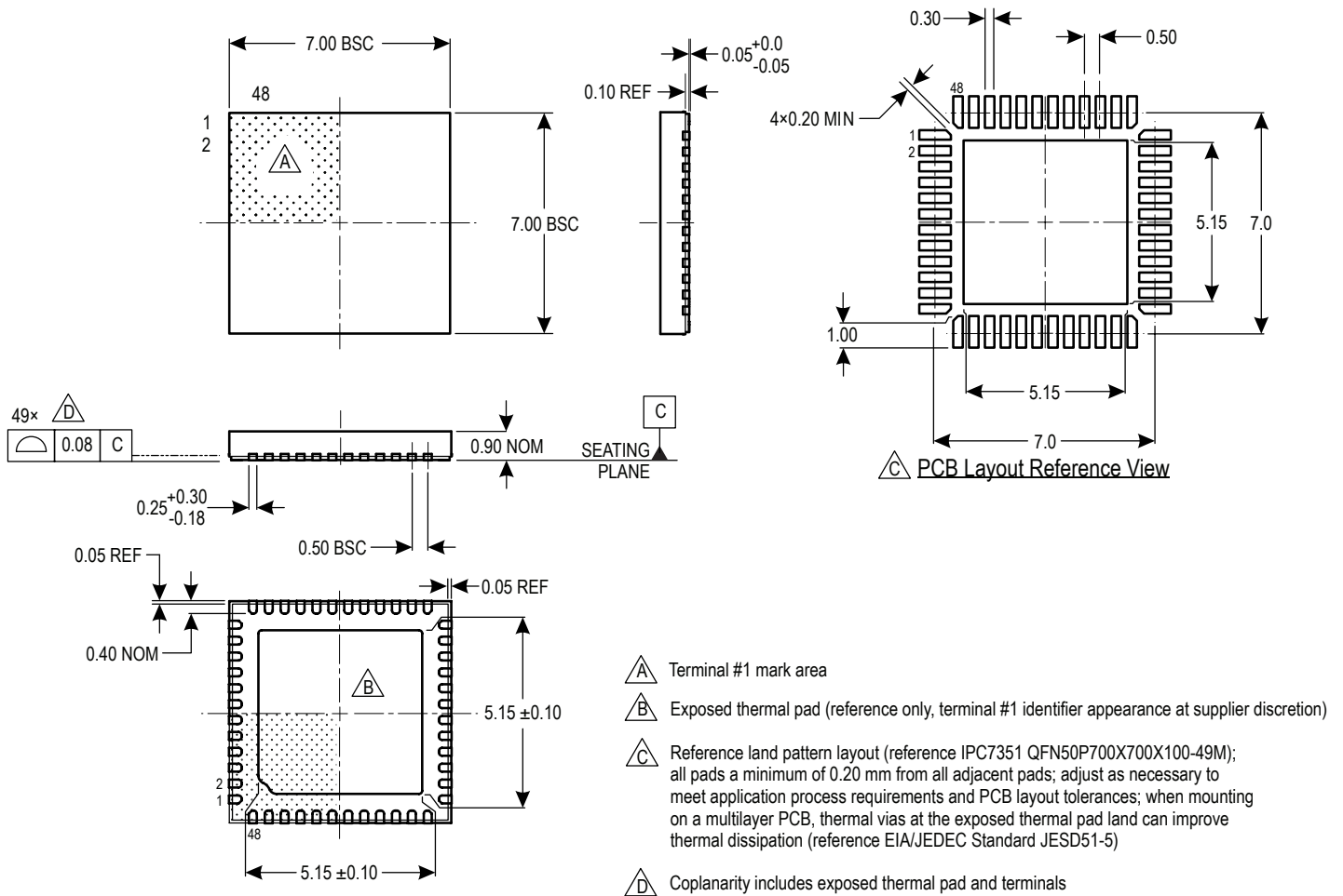
Figure 5: Package EV, 48 Terminal Wettable Flank QFN with Exposed Thermal Pad
