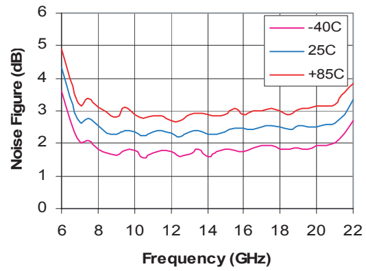
Figure 16a. Noise Figure Over Temp
