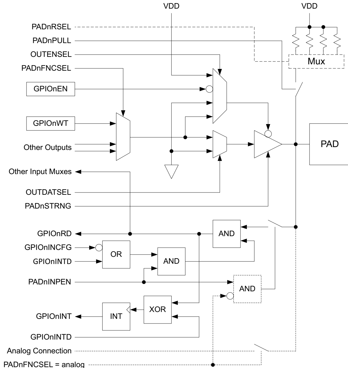
Figure 48. Pad Connection Details
