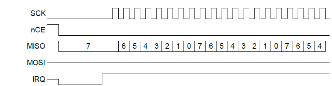
Figure 25. Flow Control at Beginning of a Raw Read Transfer
