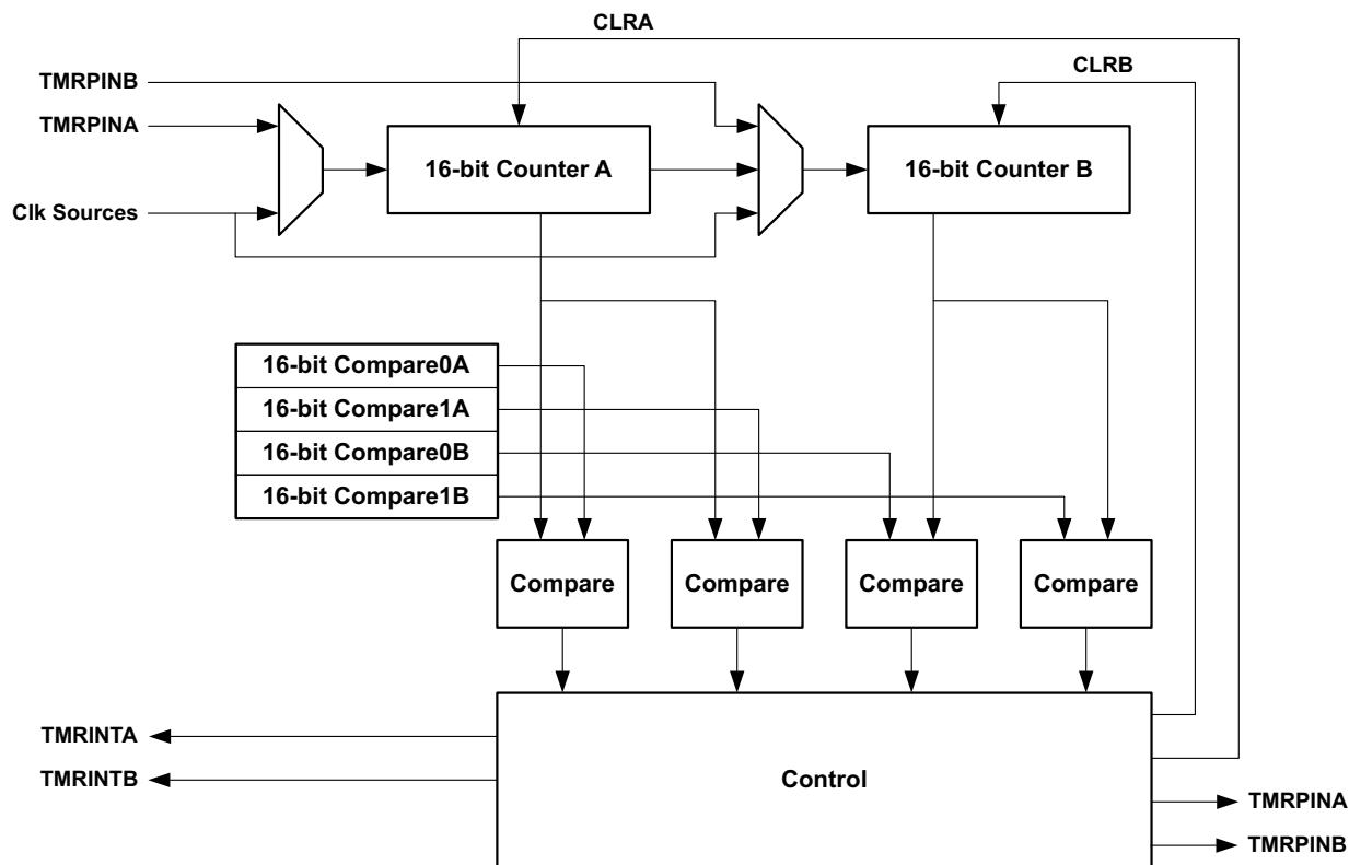
Figure 51. Block Diagram for One General Purpose Counter/Timer Pair
