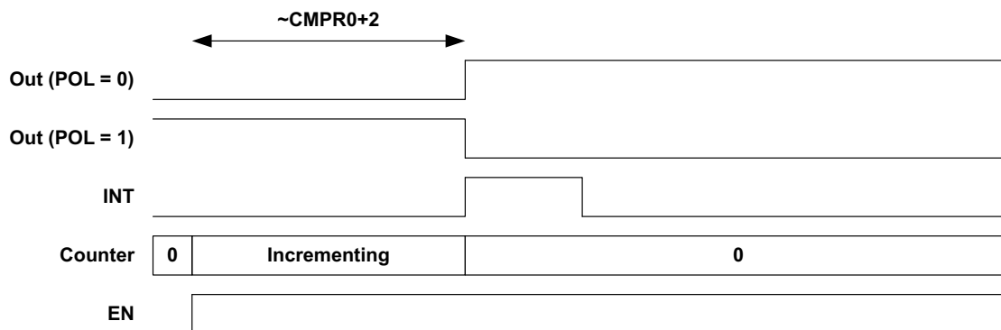
Figure 52. Counter/Timer Operation, FN = 0
