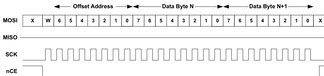
Figure 18. SPI Normal Write Operation (Single-byte Offset Address)
