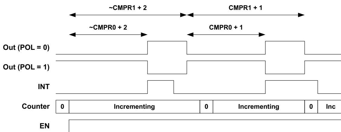
Figure 55. Counter/Timer Operation, FN = 3
