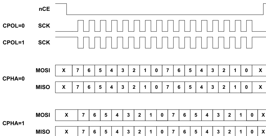
Figure 40. SPI CPOL and CPHA
