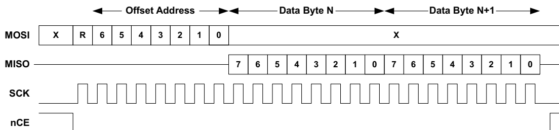
Figure 39. SPI Read Operation
