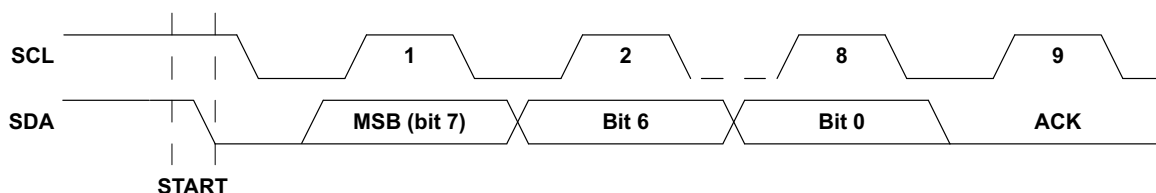
Figure 32. I 2 C Acknowledge
