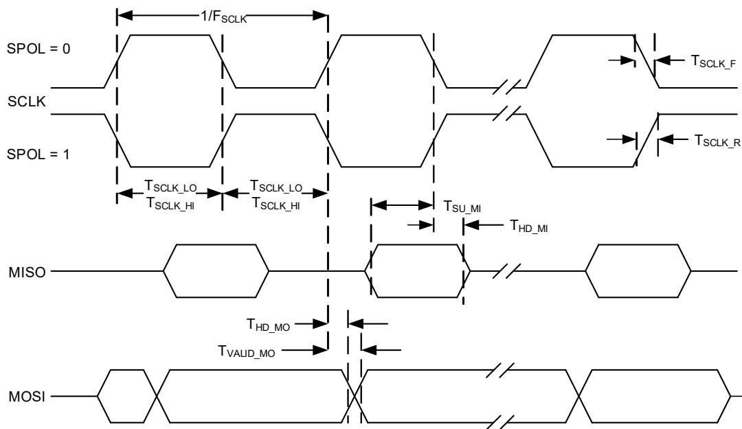
Figure 73. SPI Master Mode, Phase = 1
