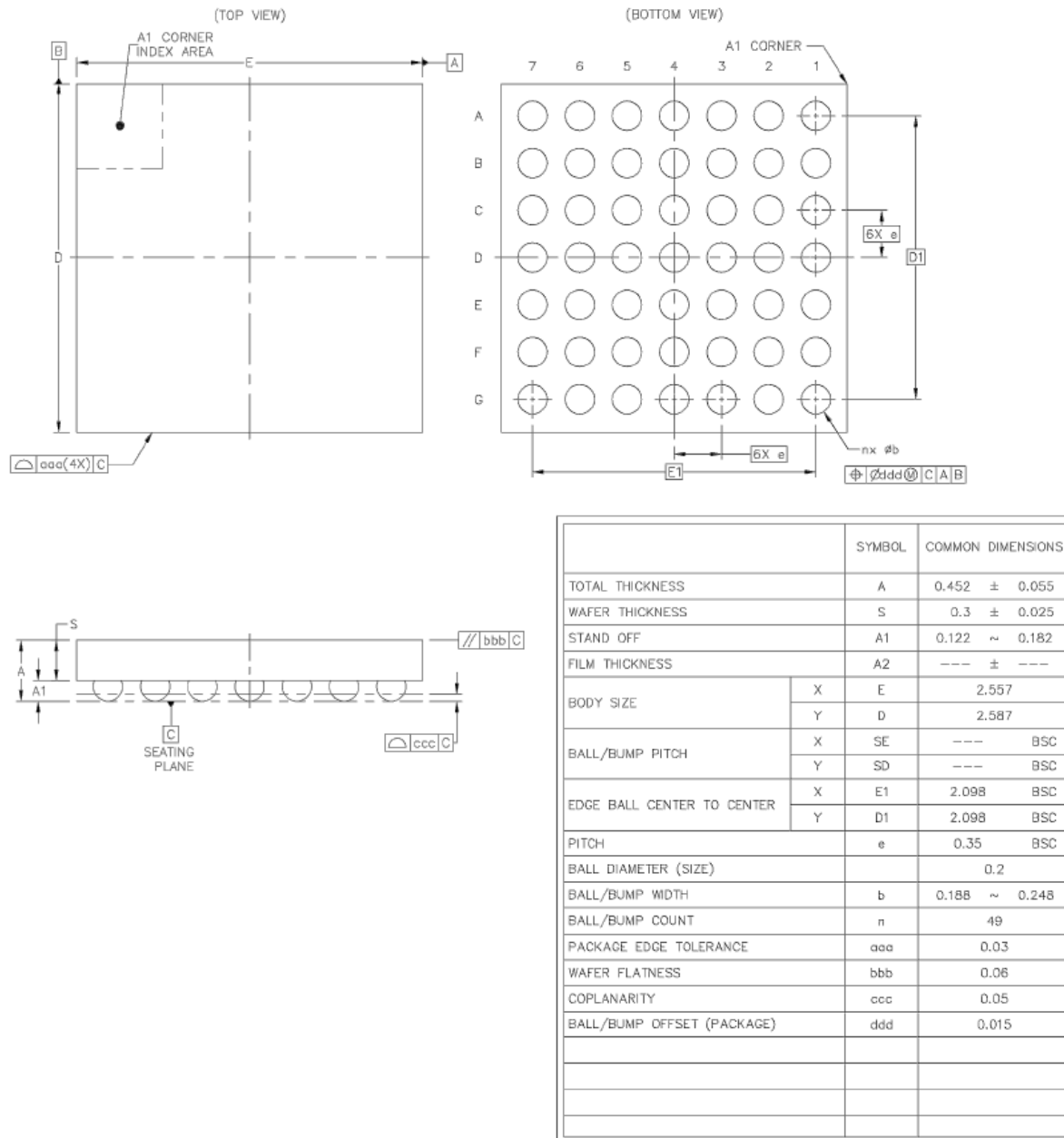
Figure 78. CSP Package Drawing
