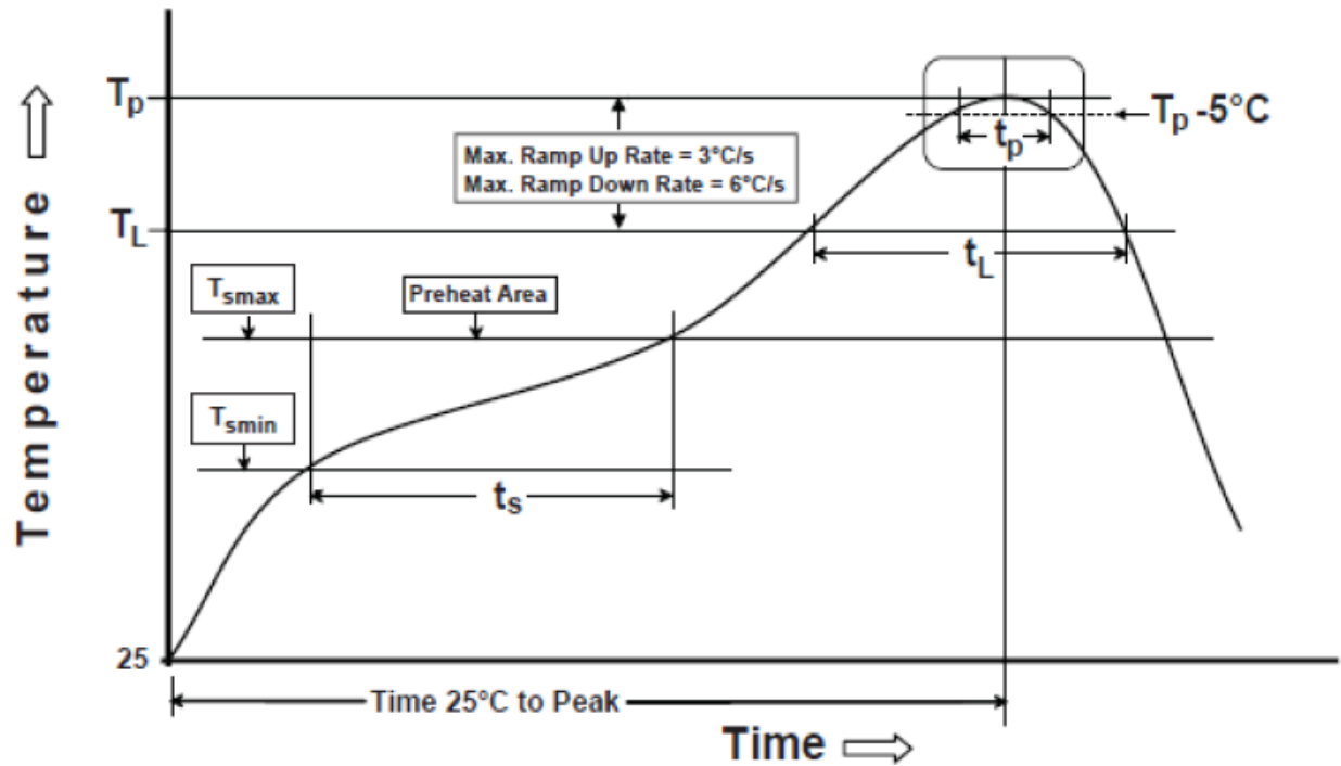
Figure 82. Reflow Soldering Diagram
