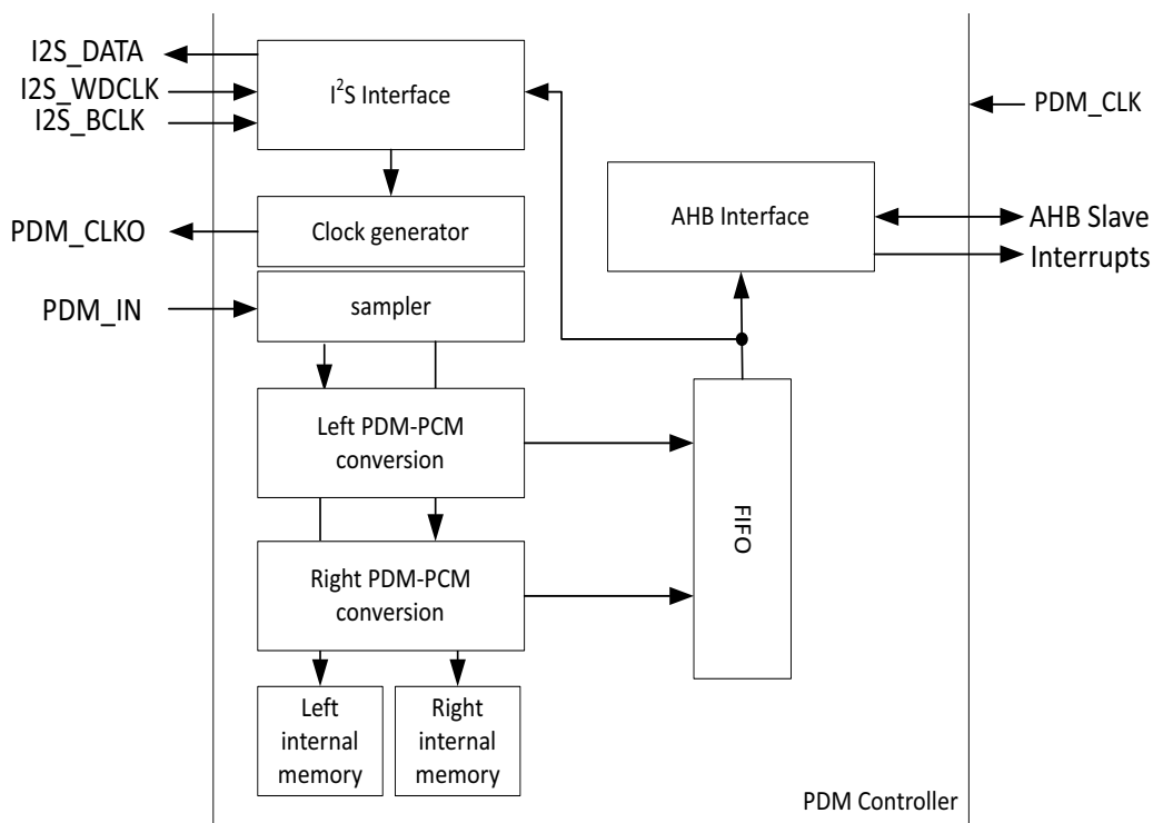
Figure 41. Block Diagram for PDM Module
