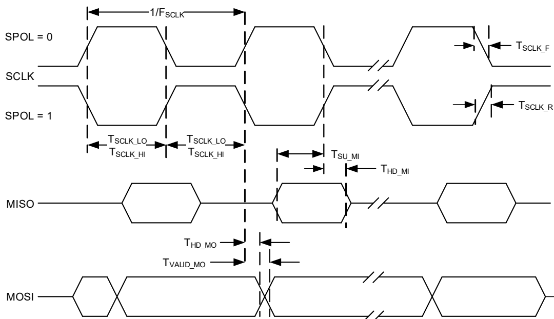
Figure 71. SPI Master Mode, Phase = 1
