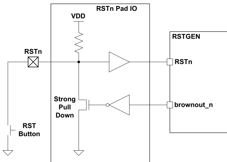
Figure 60. Block diagram of circuitry for Reset pin
