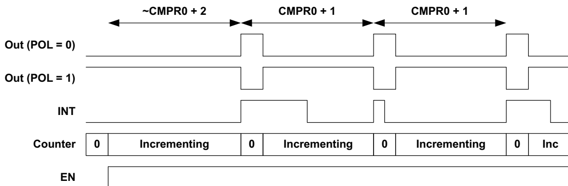
Figure 53. Counter/Timer Operation, FN = 1
