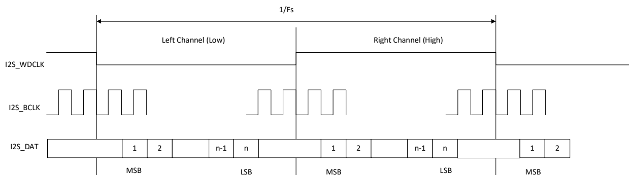
Figure 45. I 2 S Interface Data Format Timing
