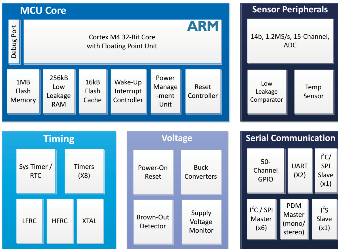
Figure 3. Block Diagram for the Ultra-Low Power Apollo2 MCU
