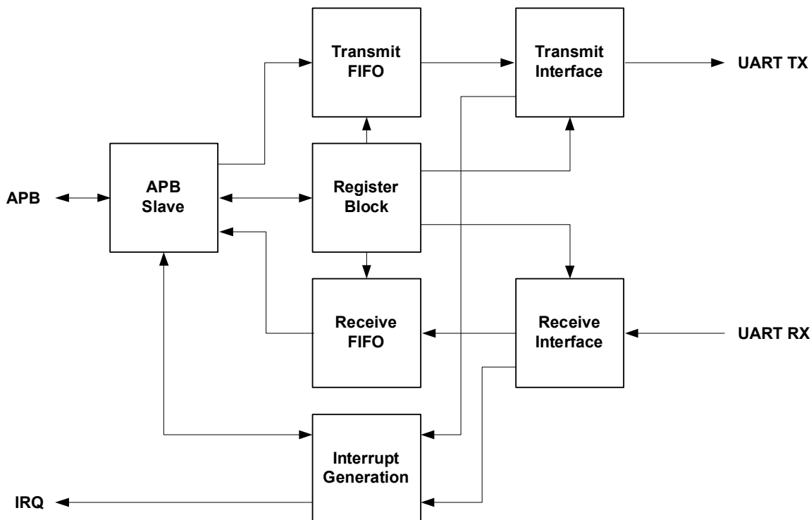
Figure 61. Block Diagram for the UART Module
