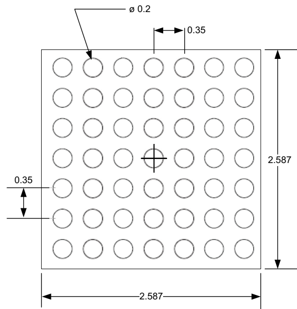
Figure 79. Land Pattern for CSP Package
