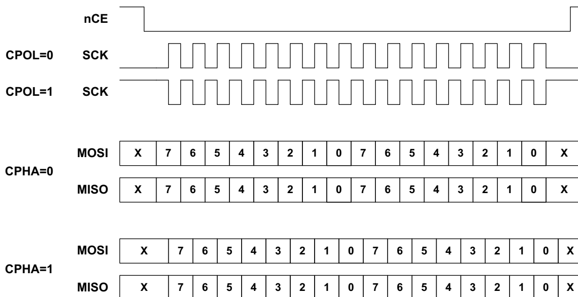
Figure 23. SPI CPOL and CPHA
