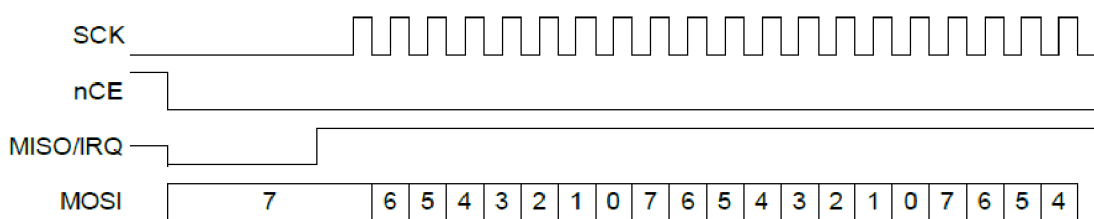
Figure 24. Flow Control at Beginning of a Write Transfer
