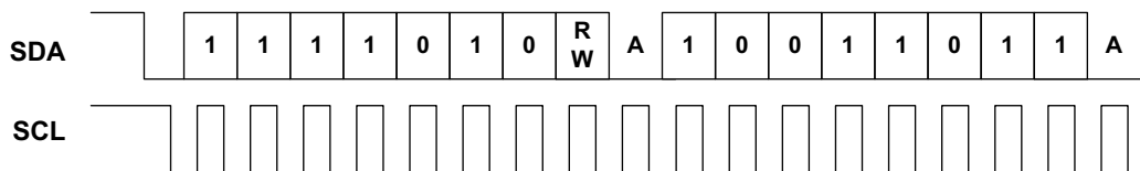
Figure 34. I 2 C 10-bit Address Operation
