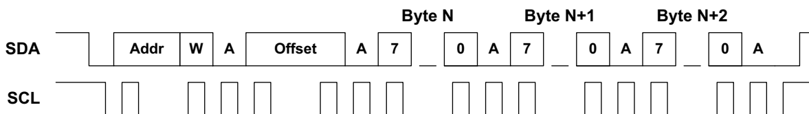
Figure 36. I 2 C Write Operation
