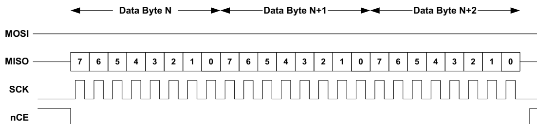
Figure 21. SPI Raw Read Operation
