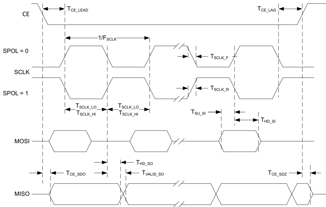
Figure 74. SPI Slave Mode, Phase = 0
