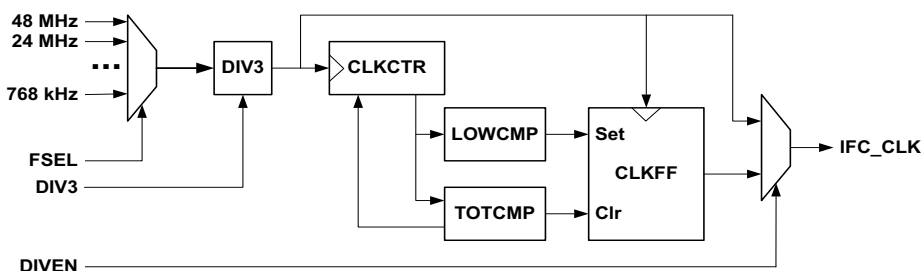
Figure 8. I 2 C/SPI Master Clock Generation
