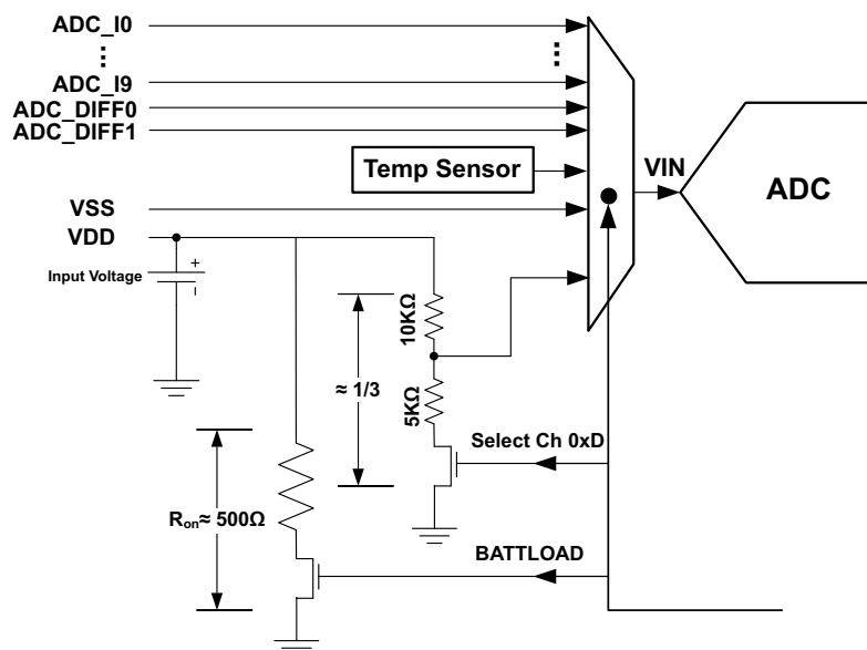
Figure 65. Switchable Battery Load
