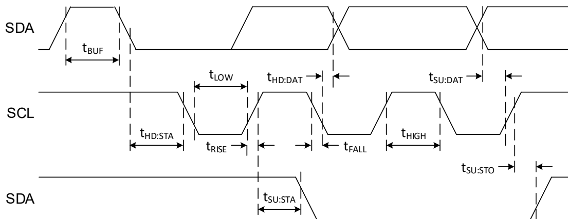
Figure 69. I 2 C Timing
