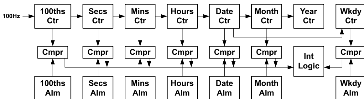
Figure 50. Block diagram for the Real Time Clock Module
