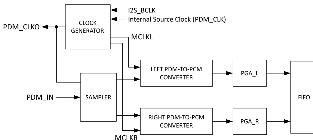
Figure 42. Stereo PDM to PCM Conversion Path
