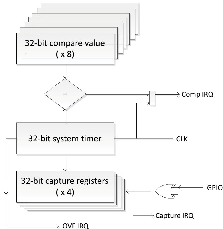
Figure 57. Block Diagram for the System Timer
