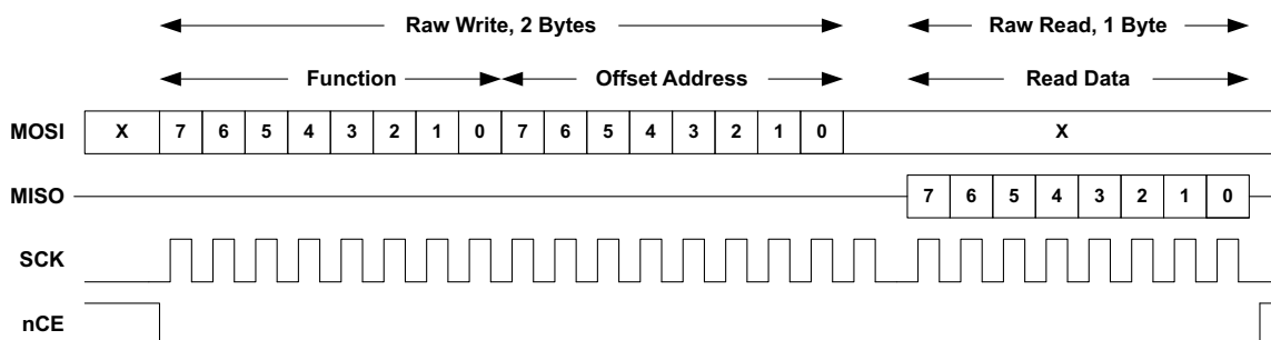
Figure 22. SPI Combined Operation
