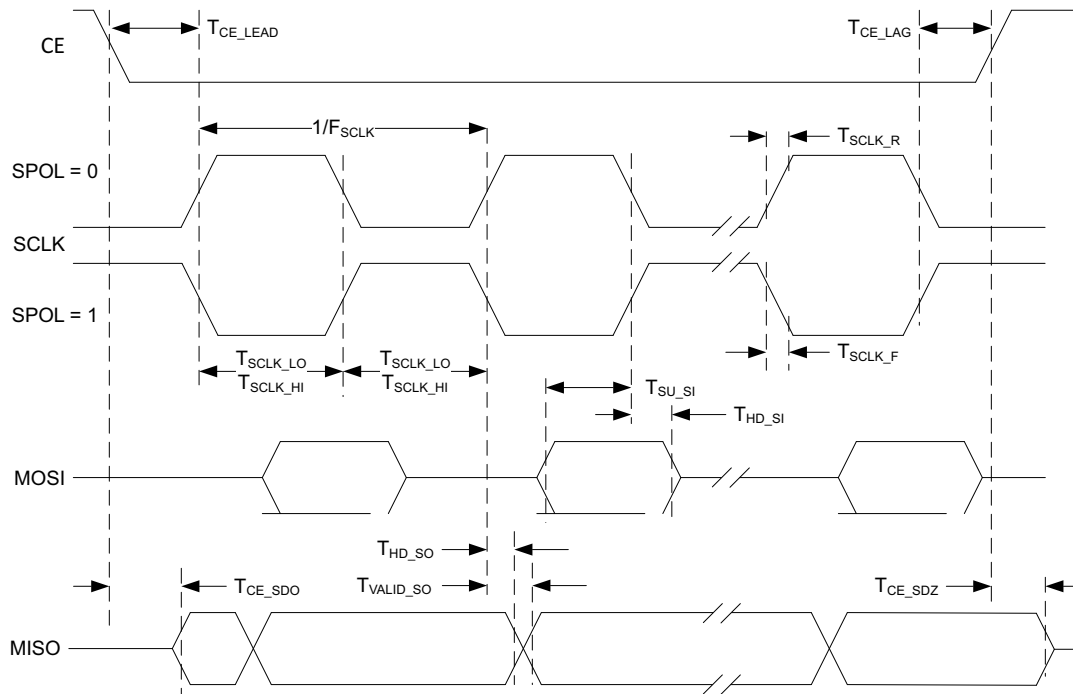
Figure 75. SPI Slave Mode, Phase = 1
