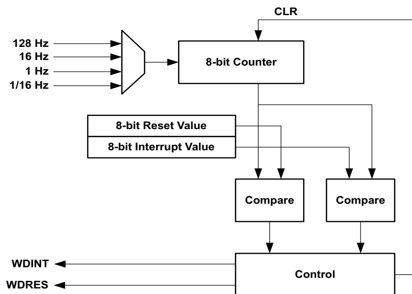
Figure 58. Block diagram for the Watchdog Timer Module
