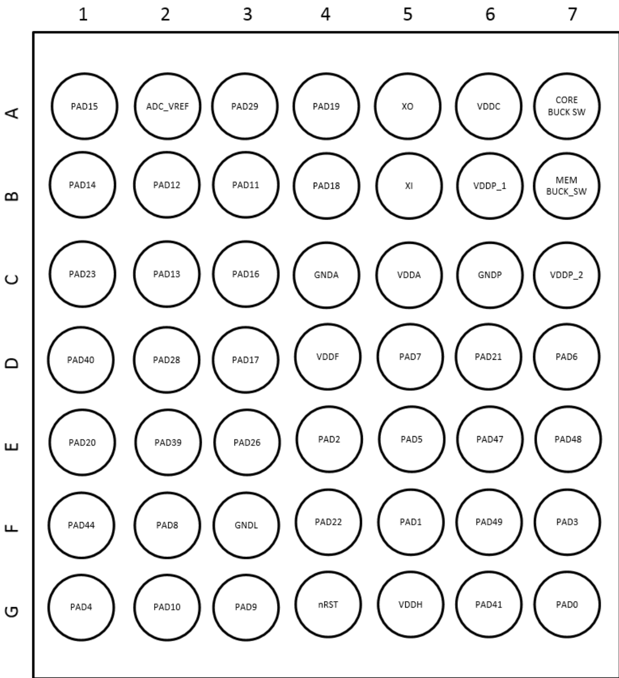
Figure 1. CSP Pin Configuration Diagram (Top View — Balls on Bottom)
