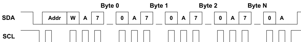
Figure 16. I 2 C Raw Write Operation
