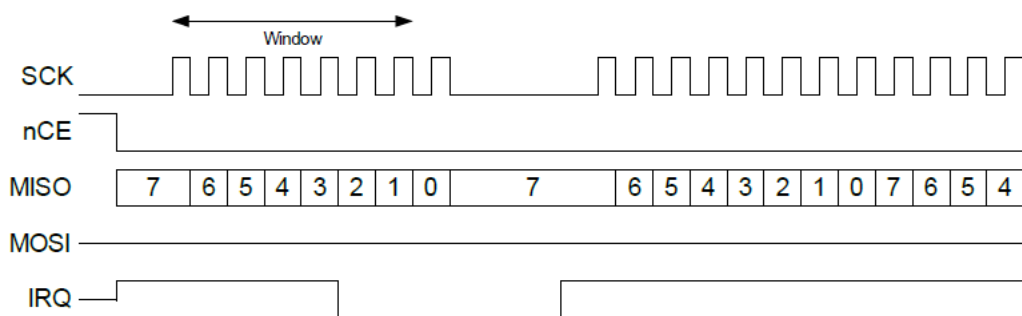
Figure 27. Flow Control in the Middle of a Read Transfer
