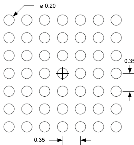
Figure 80. Example Solder Stencil Pattern for CSP Package
