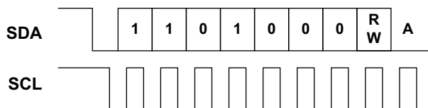
Figure 33. I 2 C 7-bit Address Operation
