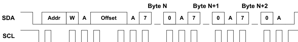
Figure 14. I 2 C Normal Write Operation
