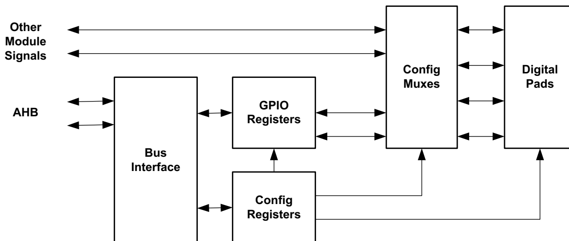
Figure 47. Block diagram for the General Purpose I/O (GPIO) Module
