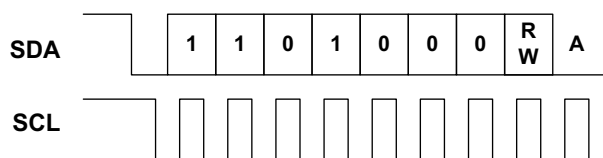
Figure 11. I 2 C 7-bit Address Operation
