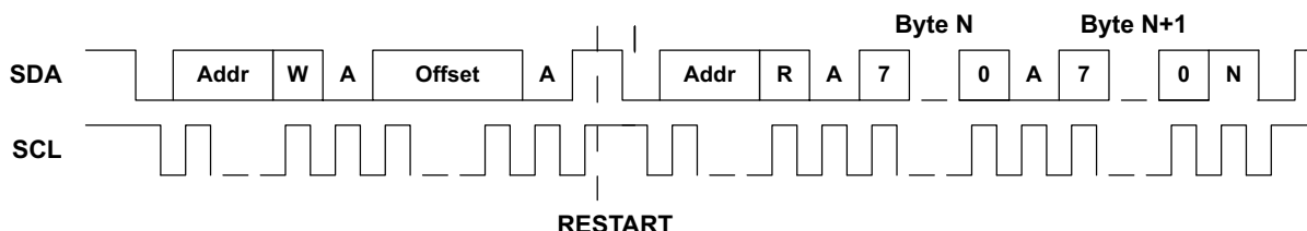
Figure 15. I 2 C Normal Read Operation
