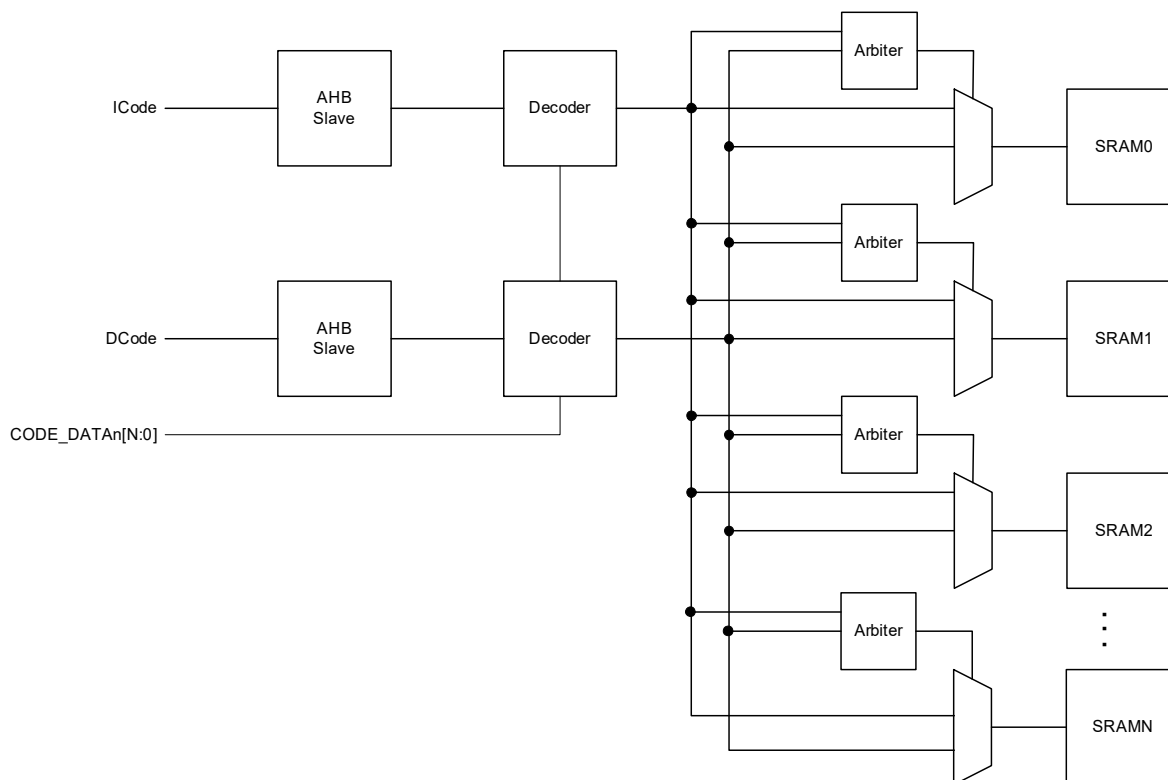
Figure 6. Block diagram for the SRAM Interface
