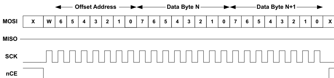
Figure 38. SPI Write Operation
