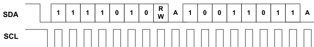
Figure 12. I 2 C 10-bit Address Operation
