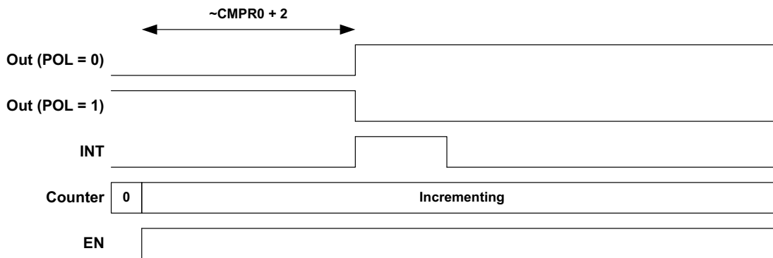
Figure 56. Counter/Timer Operation, FN = 4
