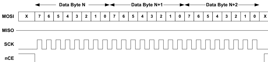
Figure 20. SPI Raw Write Operation
