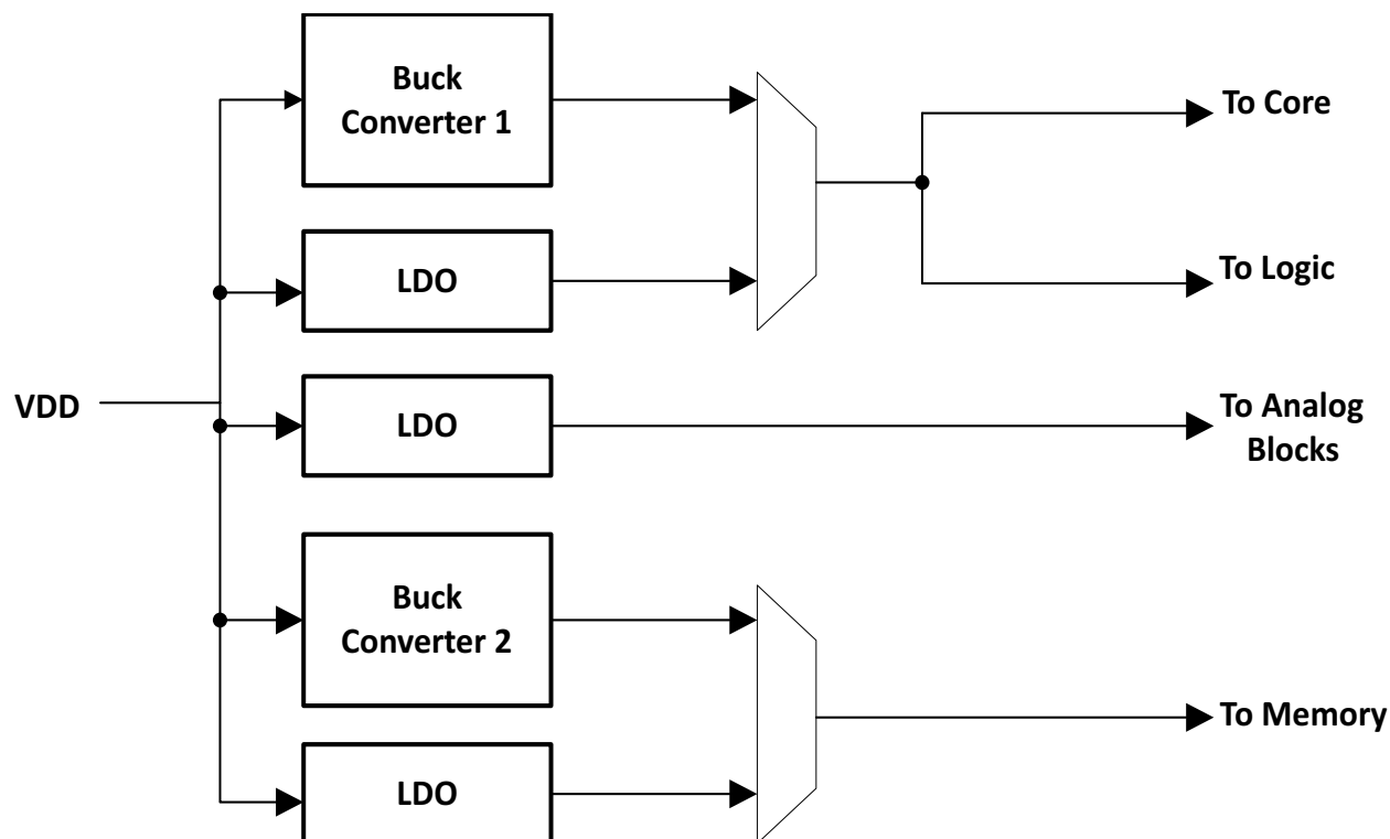
Figure 67. Block Diagram for the Voltage Regulator Module
