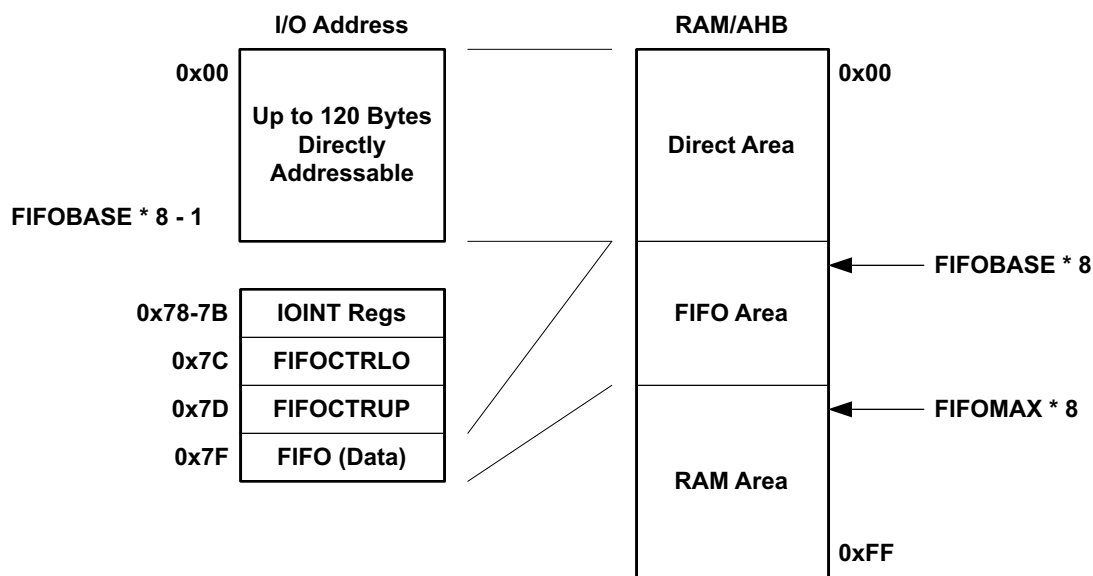
Figure 29. I 2 C/SPI Slave Module LRAM Addressing
