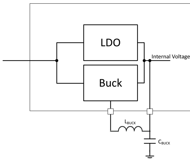
Figure 68. Buck Converter Components
