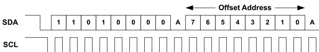
Figure 35. I 2 C Offset Address Transmission
