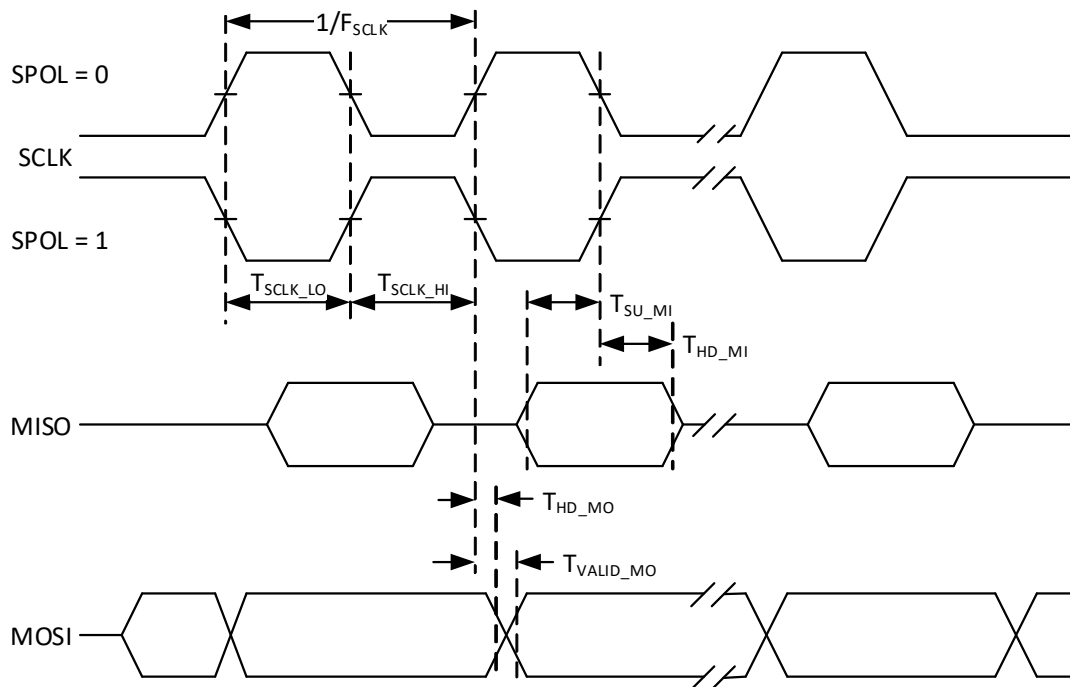
Figure 72. SPI Master Mode, Phase = 0
