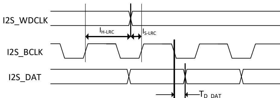
Figure 46. I 2 S Interface Setup and Hold Timing Diagram
