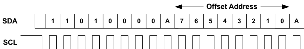
Figure 13. I 2 C Offset Address Transmission
