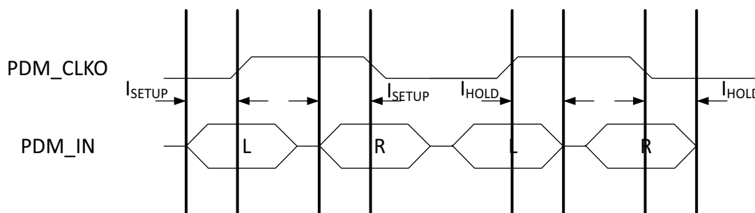
Figure 43. PDM Clock Timing Diagram
