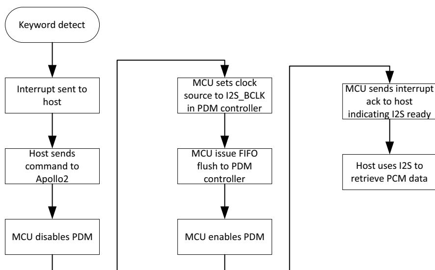
Figure 44. PDM Clock Source Switching Flow
