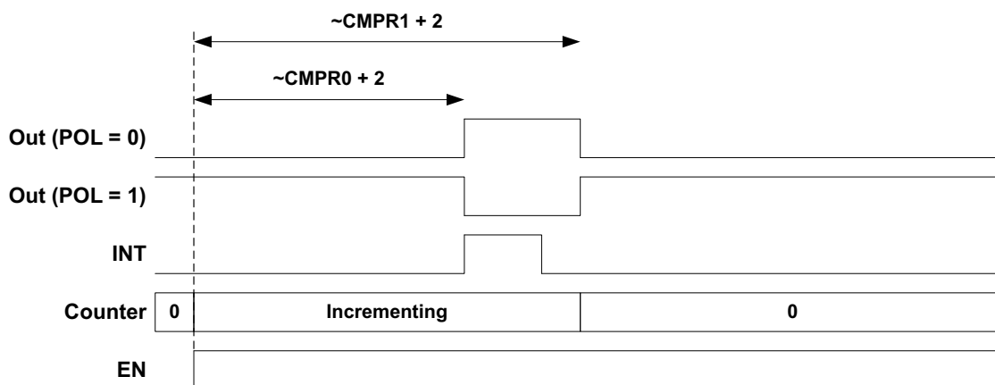
Figure 54. Counter/Timer Operation, FN = 2
