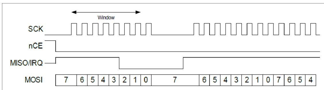
Figure 26. Flow Control in the Middle of a Write Transfer
