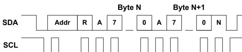
Figure 17. I 2 C Raw Read Operation
