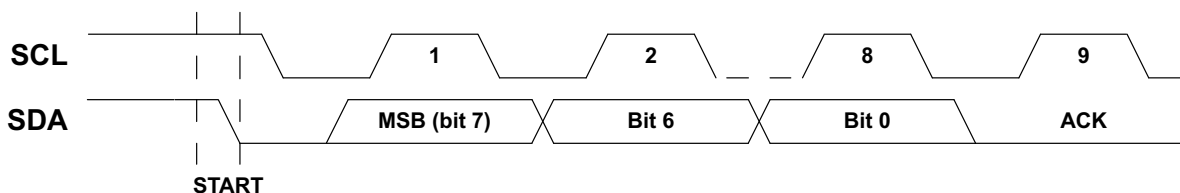
Figure 10. I 2 C Acknowledge
