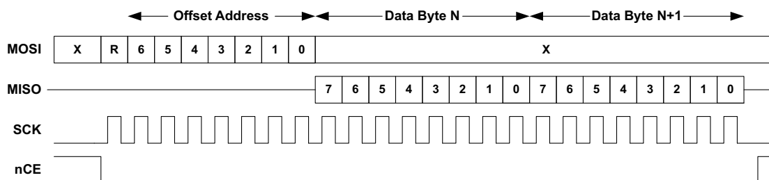
Figure 19. SPI Normal Read Operation
