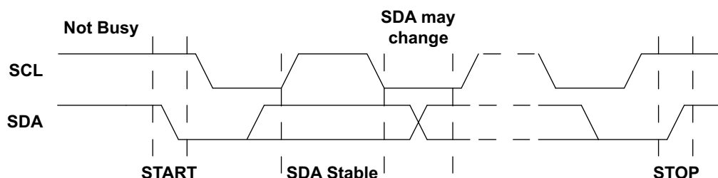
Figure 31. Basic I 2 C Conditions
