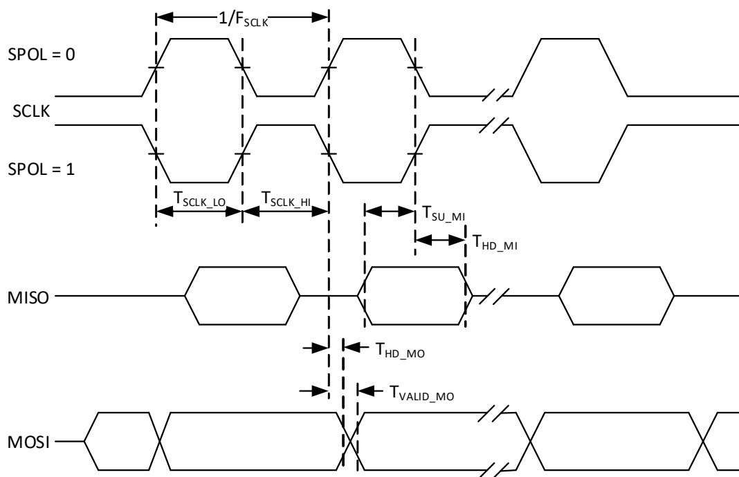
Figure 70. SPI Master Mode, Phase = 0
