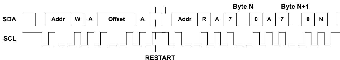
Figure 37. I 2 C Read Operation
