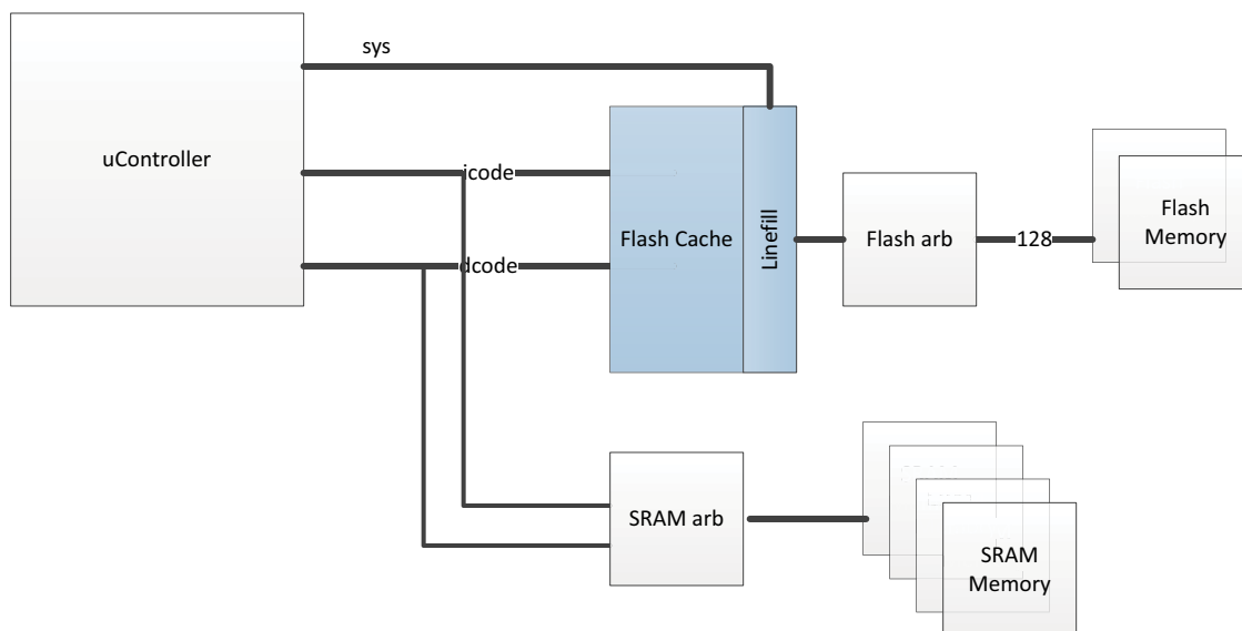
Figure 4. Block Diagram for Apollo2 MCU with Flash Cache
