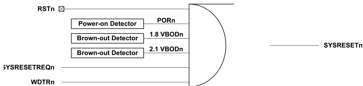
Figure 59. Block diagram for the Reset Generator Module
