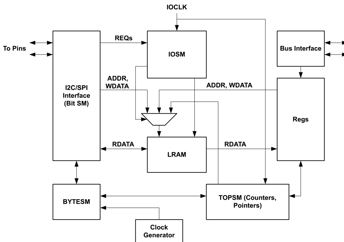
Figure 7. Block Diagram for the I 2 C/SPI Master Module
