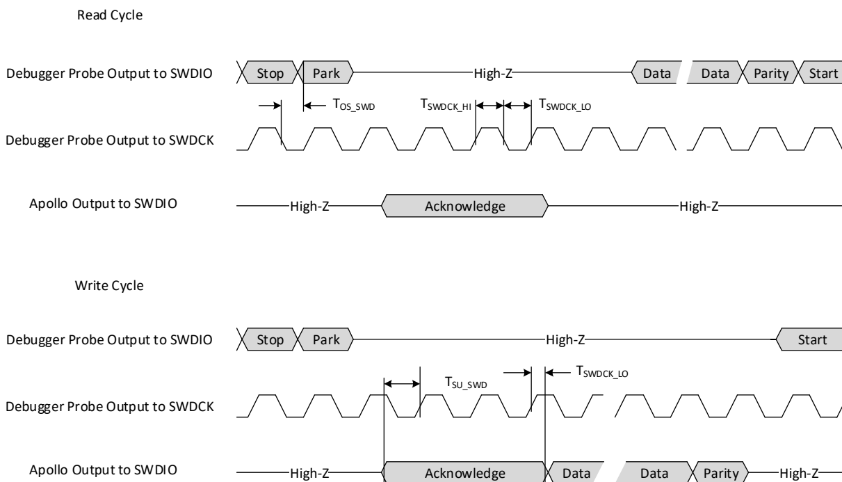
Figure 76. Serial Wire Debug Timing
